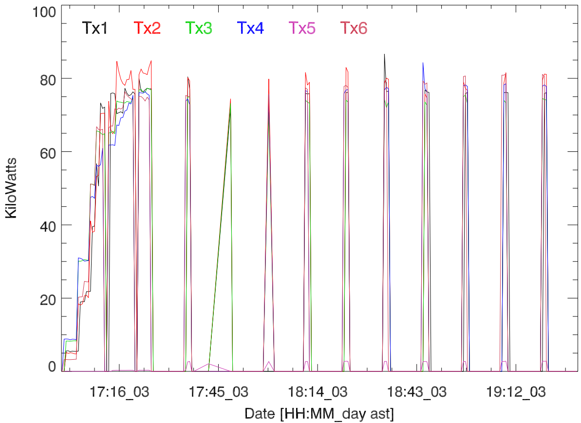
TxPwr by Tx. 03nov16:H1111. Frank & Herb.
