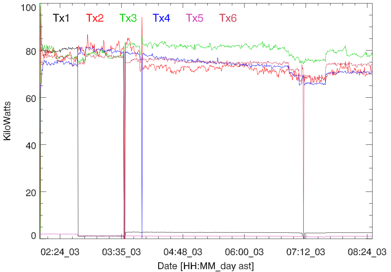
TxPwr by Tx. 03nov16:T2869. Suman Ganguly.
