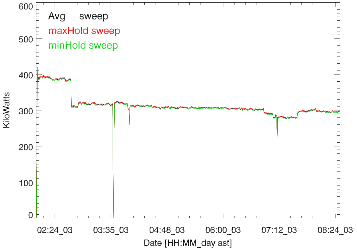
TxPwrTot. 03nov16:T2869. Suman Ganguly. 5 MHz
