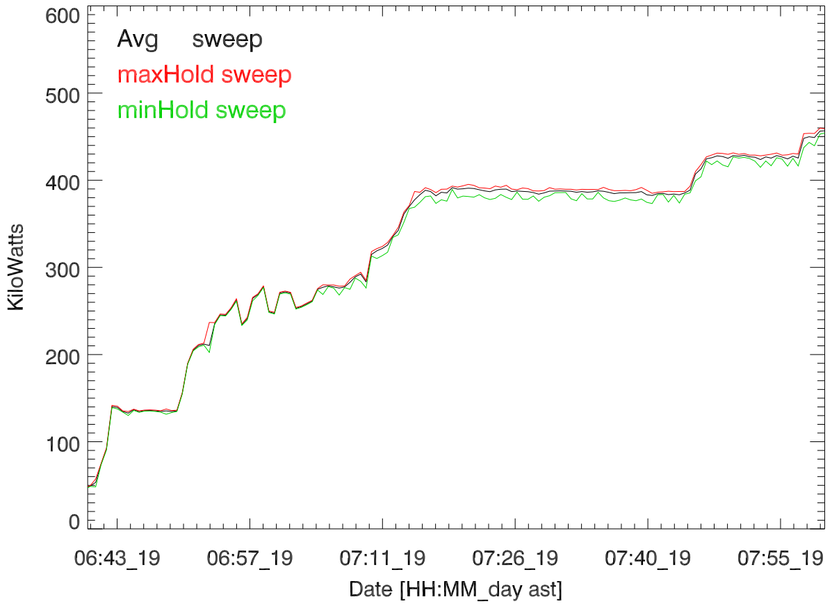
TxPwrTot. 19mar17:H3111. Frank & Herb 8 MHz
