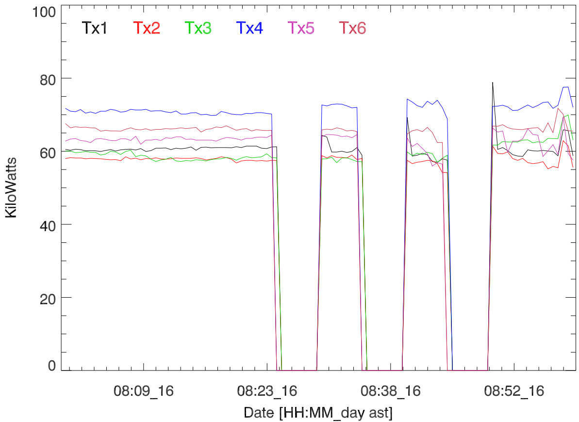
TxPwr by Tx. 16mar17:H3156. Paul Bernhardt epop
