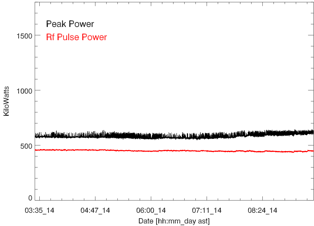
CH 430 Transmitted power for: 14mar17:T2869. Suman Ganguly.
