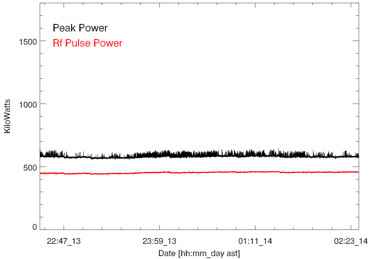
CH 430 Transmitted power for: 13mar17:T2915. Salih Boston.
