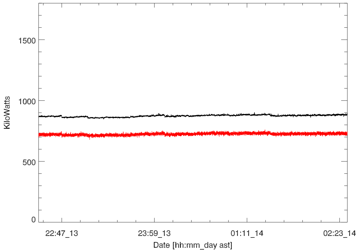
GD 430 Transmitted power for: 13mar17:T2915. Salih Boston.
