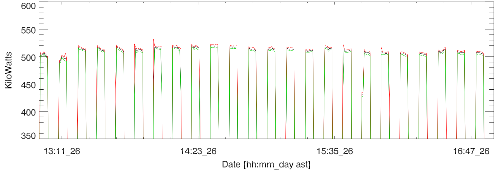
jun20 hf campaign, Transmitted power (total). 200626
