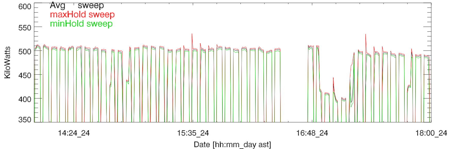
jun20 hf campaign, Transmitted power (total). 200624
