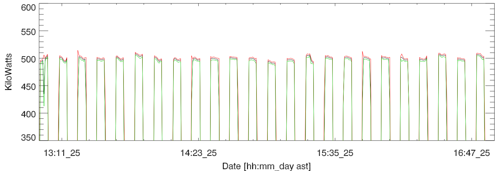
jun20 hf campaign, Transmitted power (total). 200625
