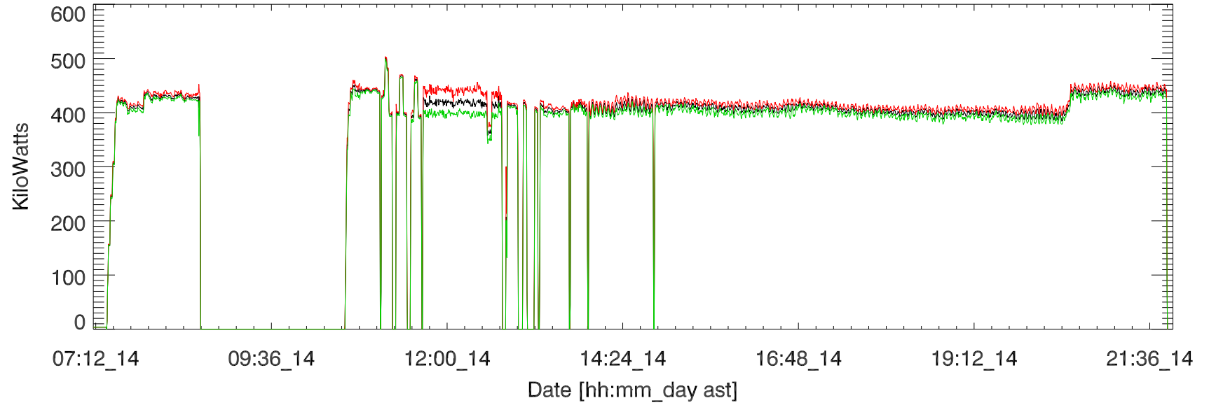
jun19 hf campaign, Transmitted power (total). 190614
