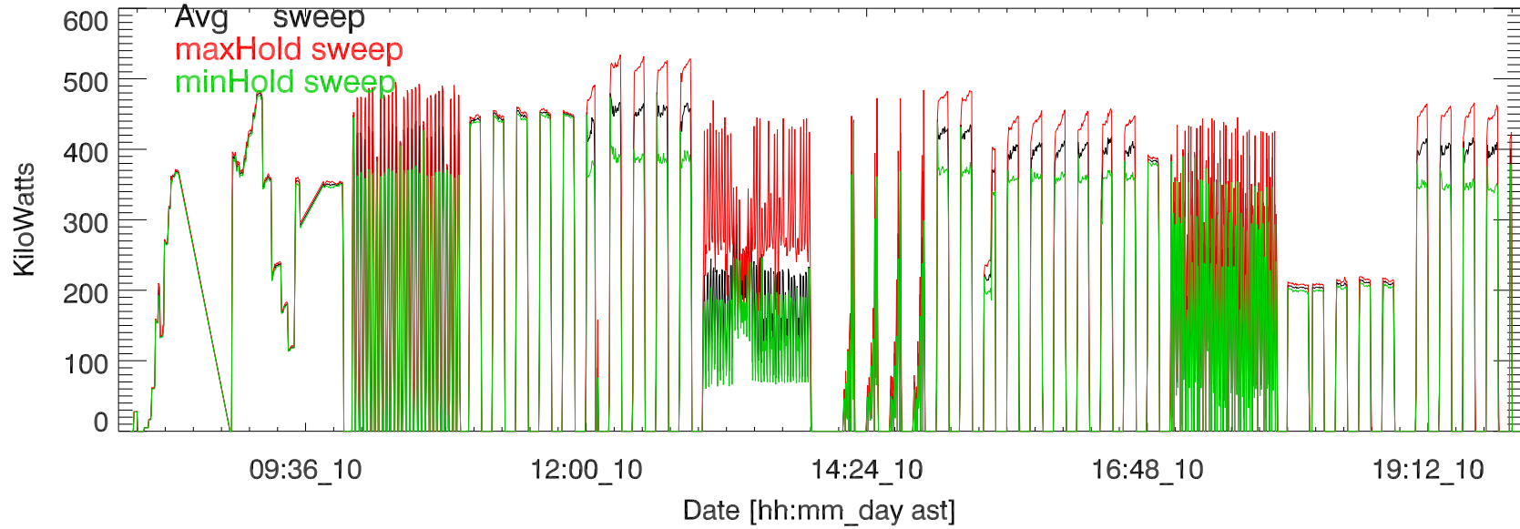
jun19 hf campaign, Transmitted power (total). 190610
