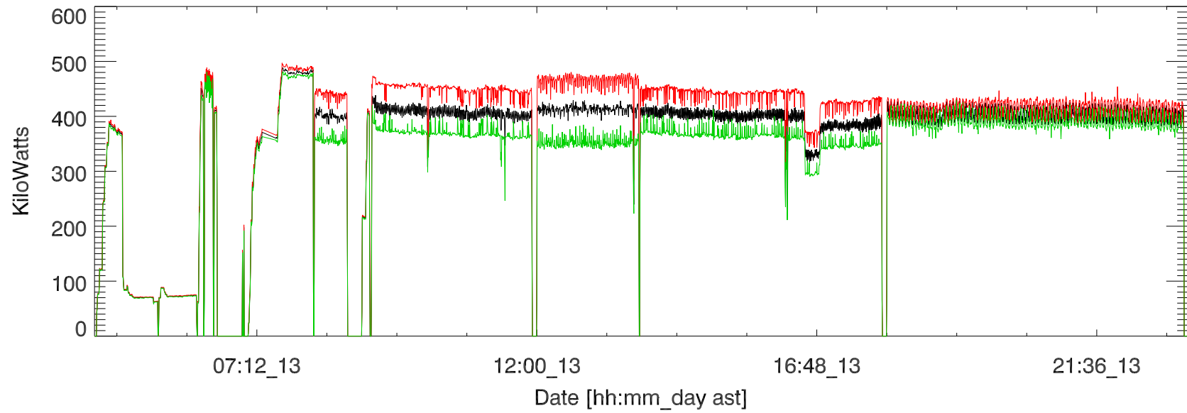
jun19 hf campaign, Transmitted power (total). 190613
