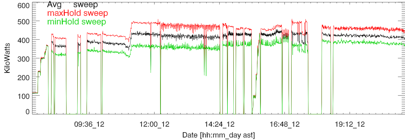
jun19 hf campaign, Transmitted power (total). 190612
