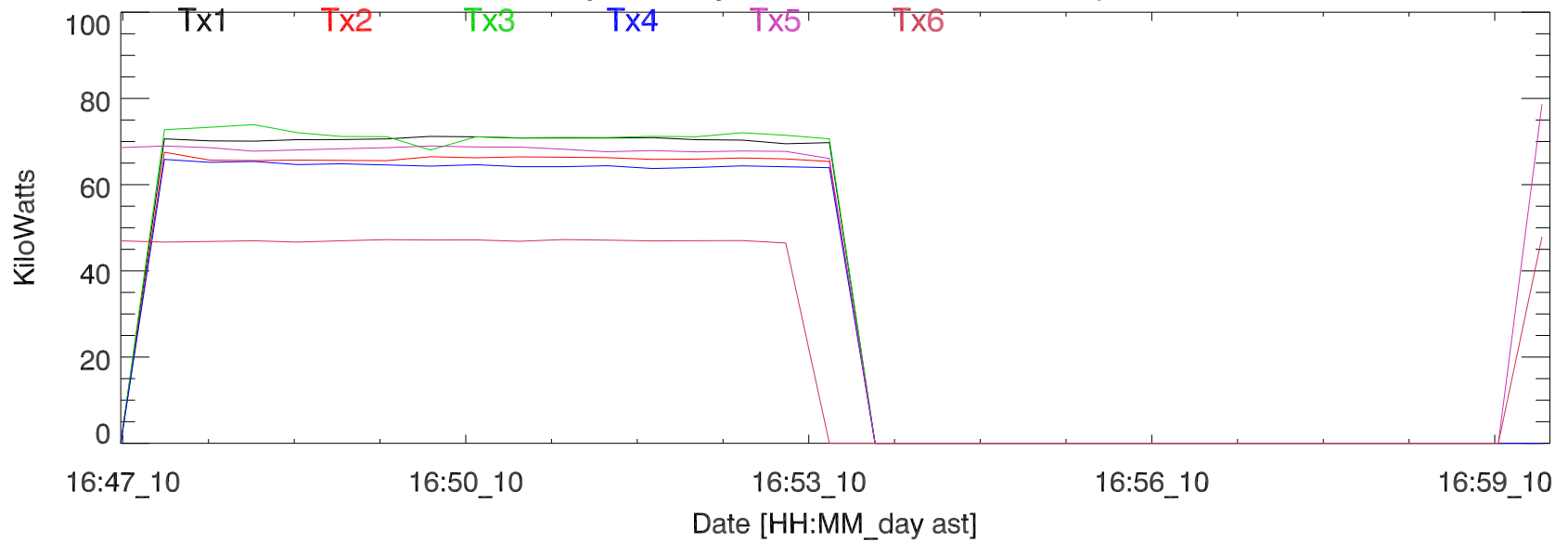
TxPwr by Tx. 10jun19:H3195 vladimir exp10.08
