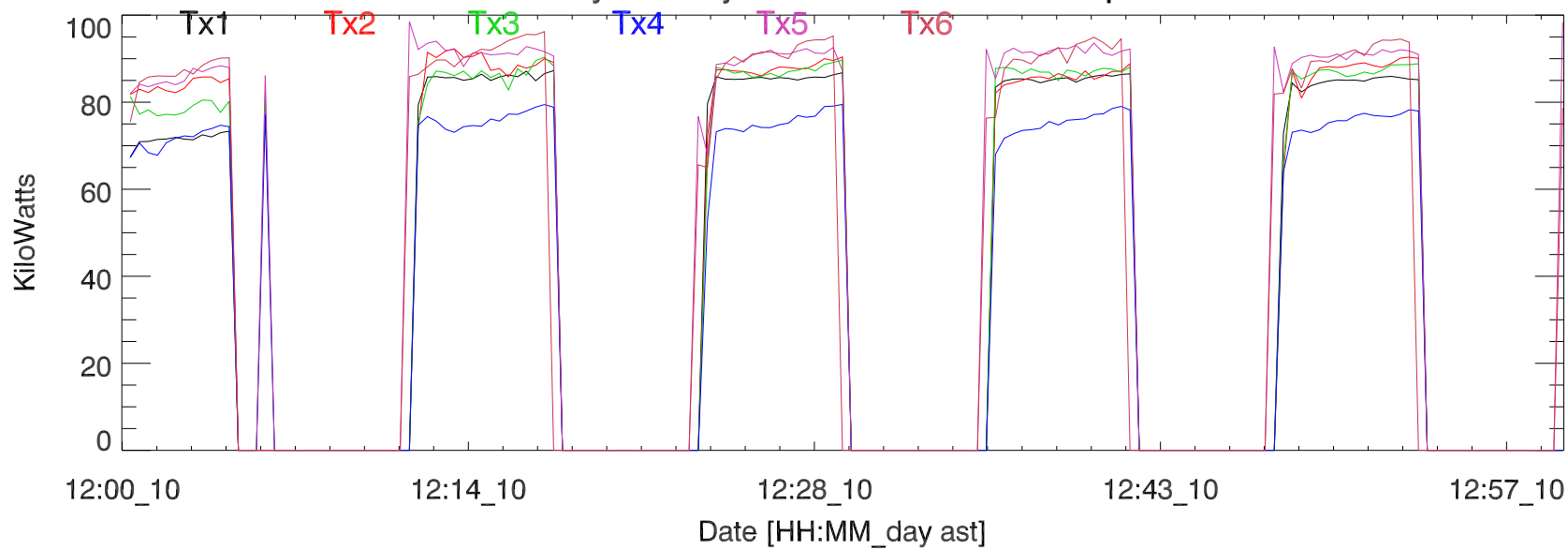
TxPwr by Tx. 10jun19:H3195 vladimir exp10.04
