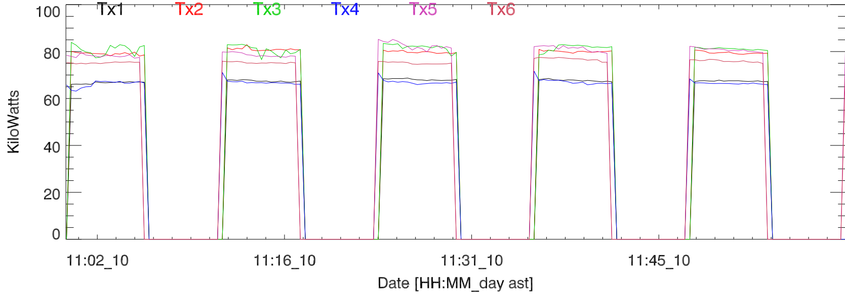
TxPwr by Tx. 10jun19:H3195 vladimir exp10.03
