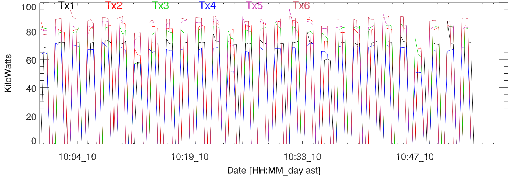
TxPwr by Tx. 10jun19:H3195 vladimir exp10.02
