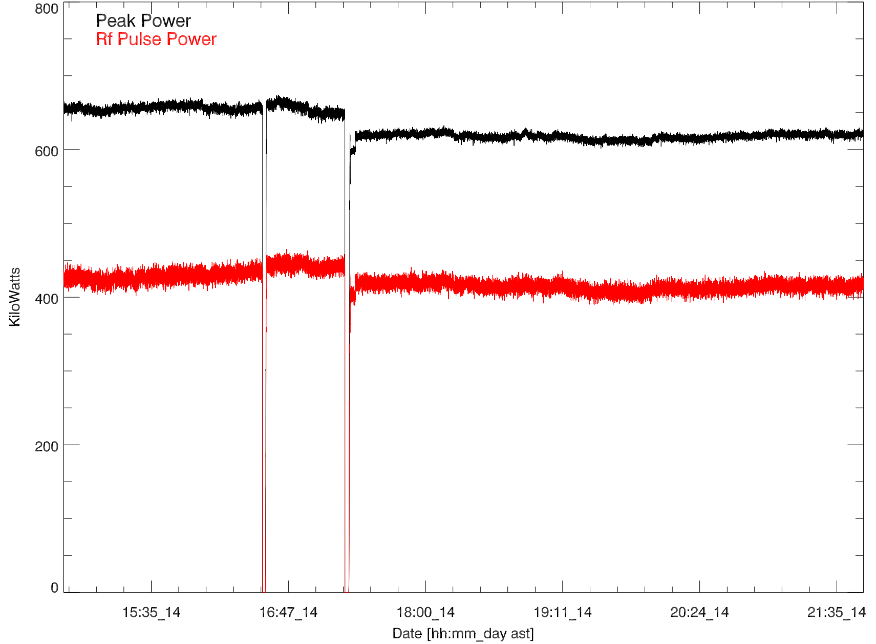
GD 430 Transmitted power for: 14jun19:H3337 paul exp14.08
