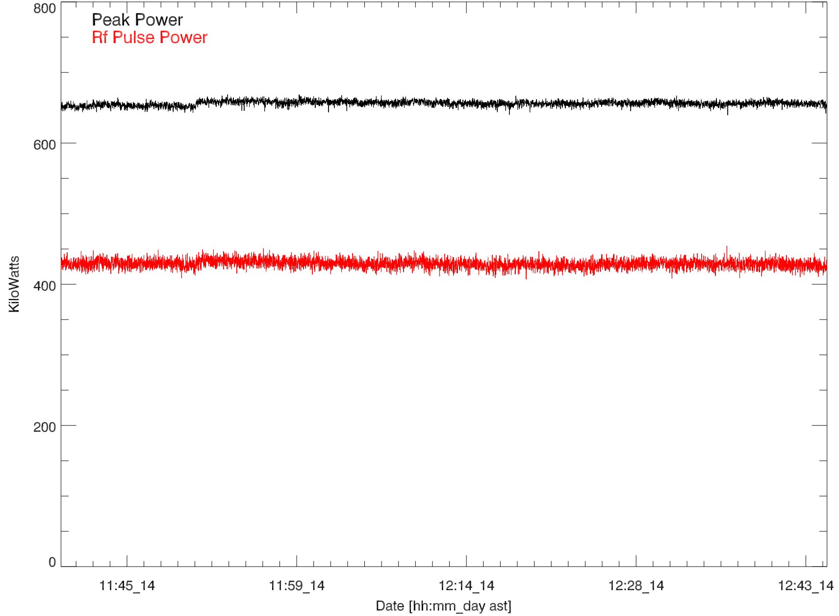
GD 430 Transmitted power for: 14jun19:H3337 paul exp14.03
