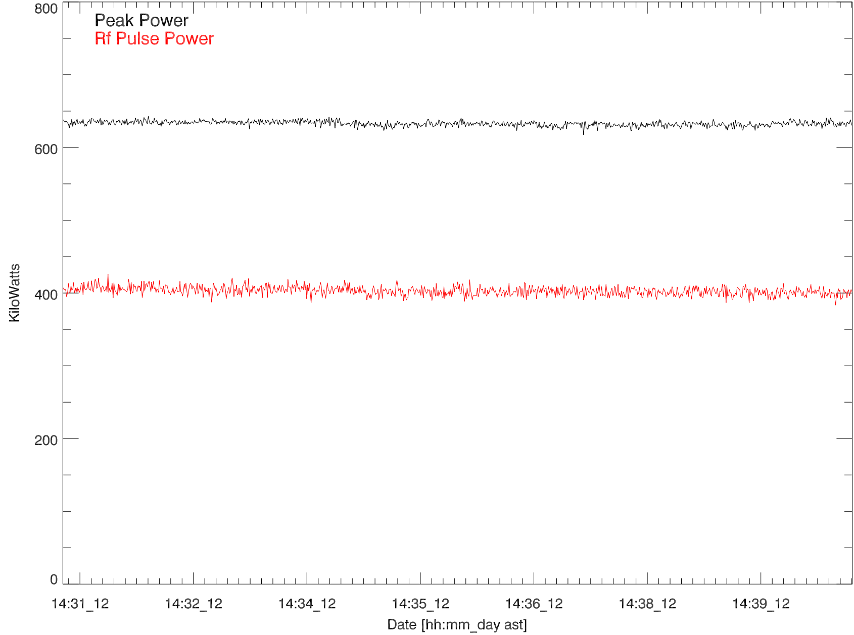
GD 430 Transmitted power for: 12jun19:H3337 paul exp12.06
