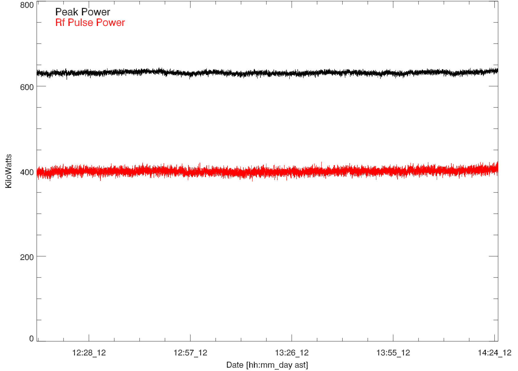
GD 430 Transmitted power for: 12jun19:H3337 paul exp12.05
