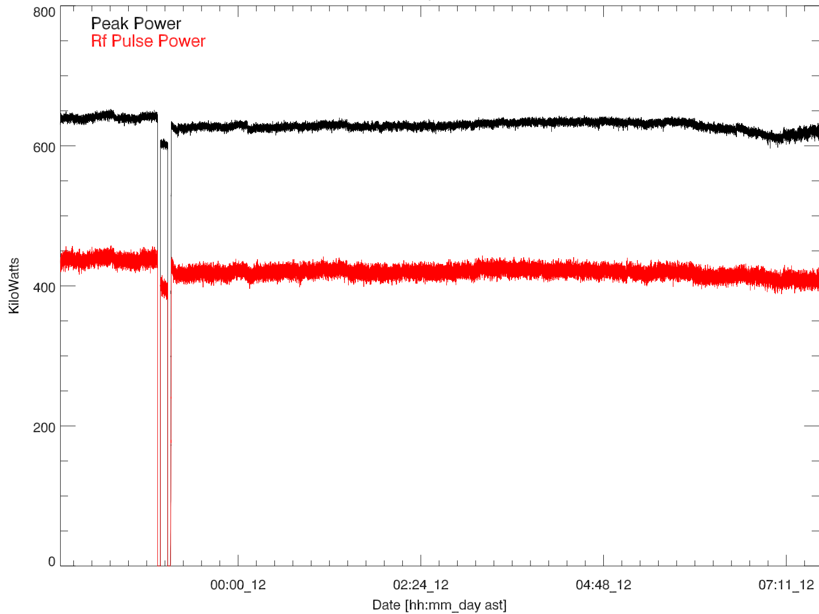
GD 430 Transmitted power for: 11jun19:T1193 suman (no hf) exp11.20
