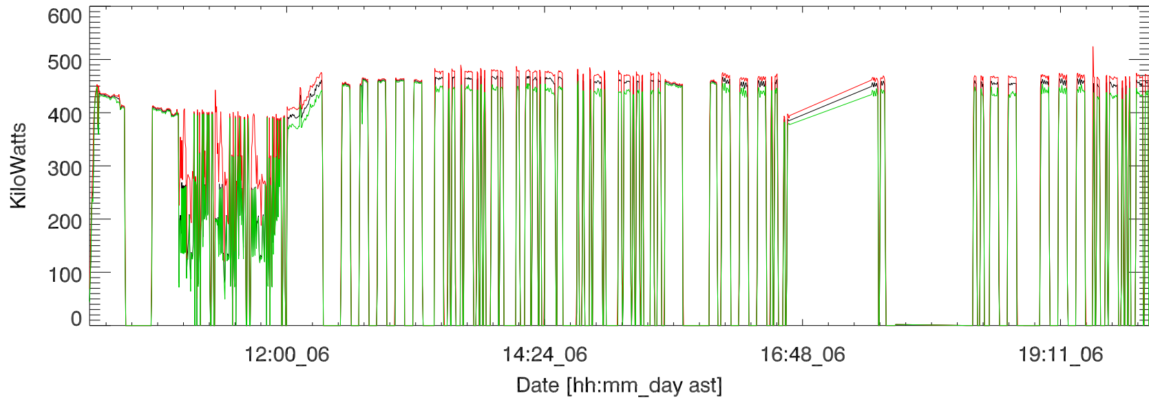
nov18 hf campaign, Transmitted power (total). 181106
