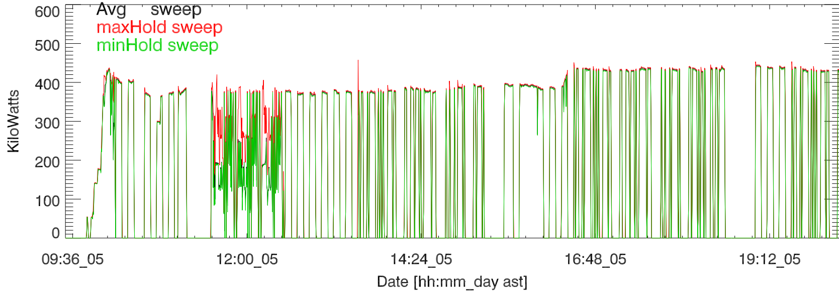
nov18 hf campaign, Transmitted power (total). 181105
