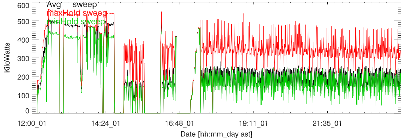
nov18 hf campaign, Transmitted power (total). 181101
