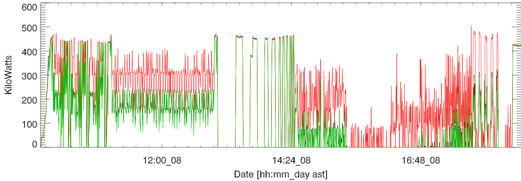
nov18 hf campaign, Transmitted power (total). 181108
