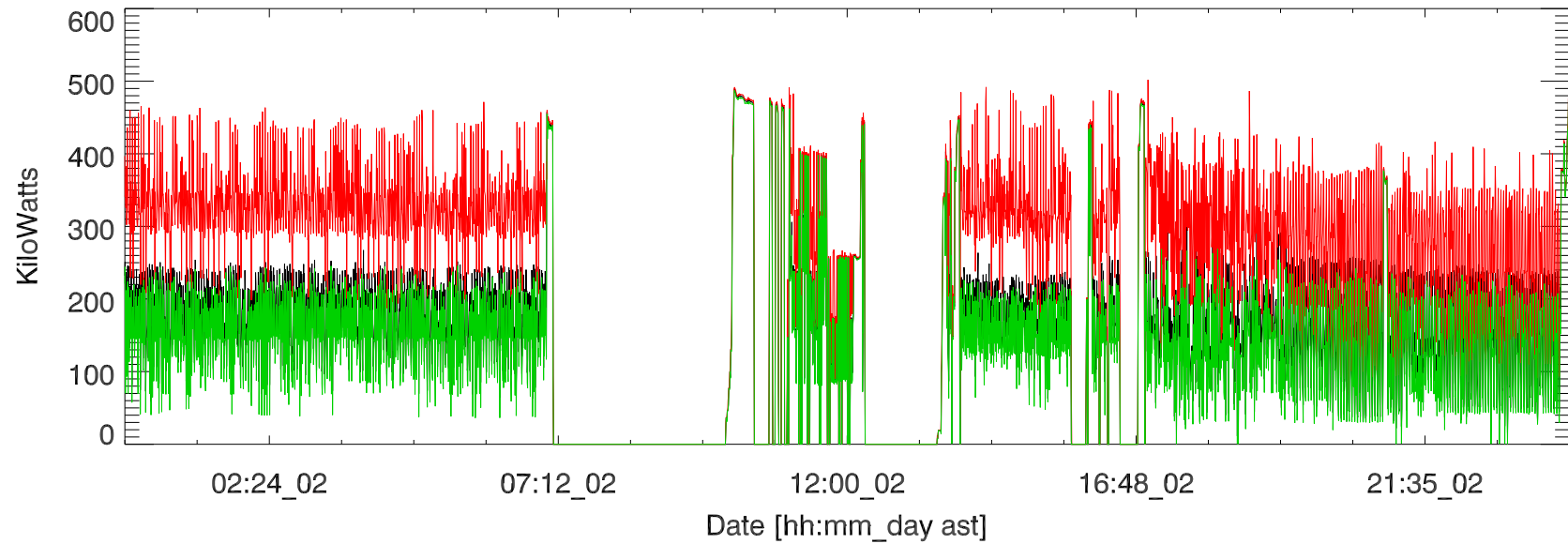
nov18 hf campaign, Transmitted power (total). 181102
