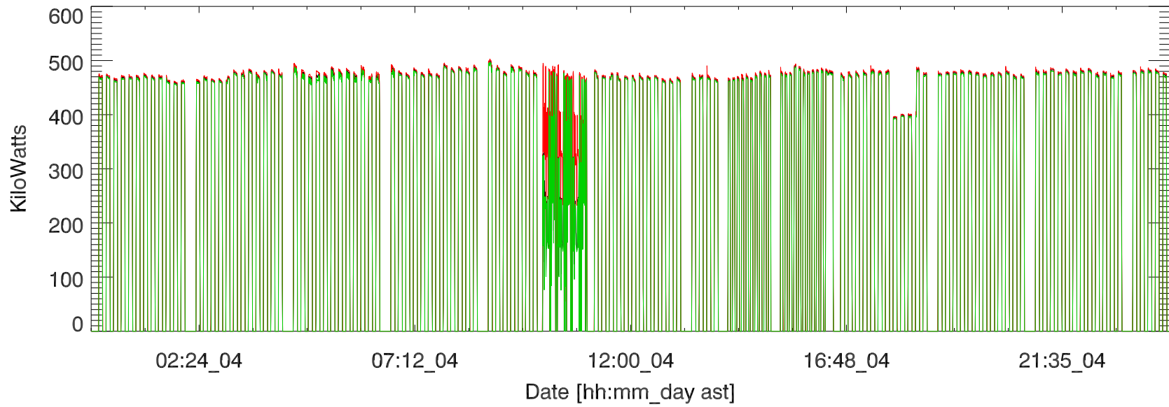
nov18 hf campaign, Transmitted power (total). 181104
