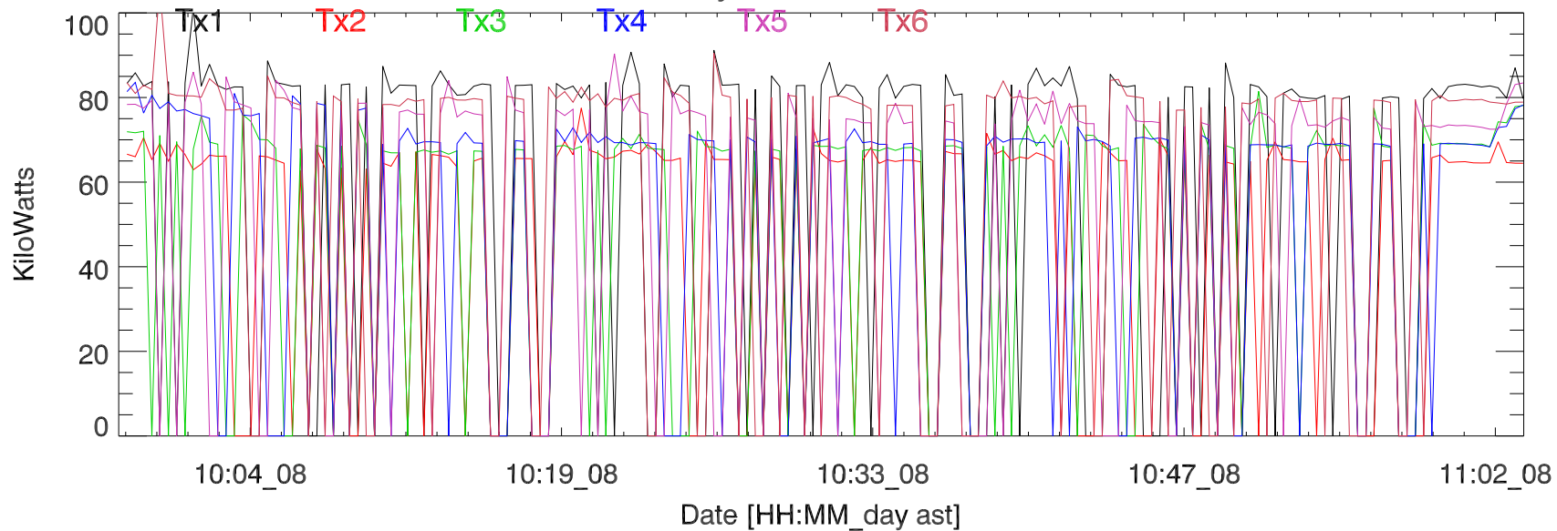
TxPwr by Tx. 08nov18:H3286
