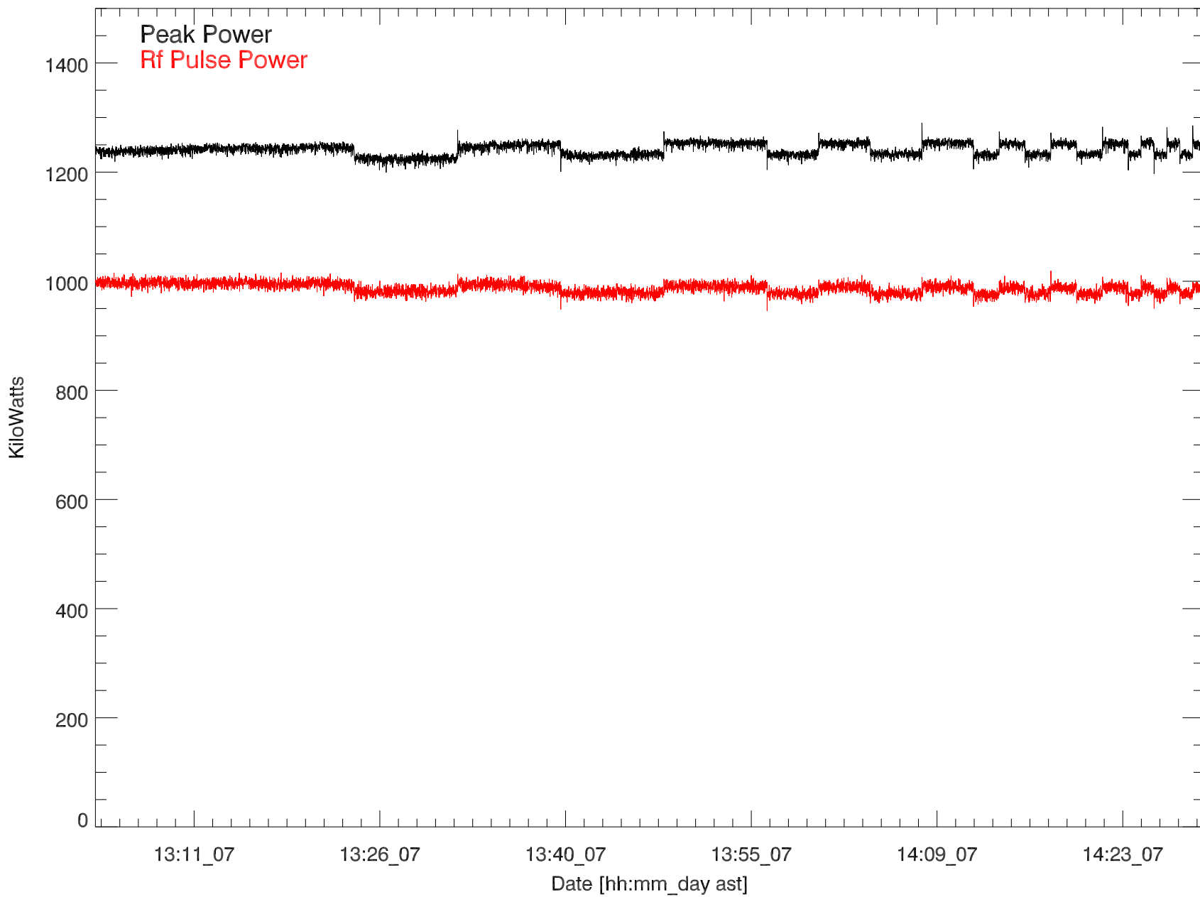
GD 430 Transmitted power for: 07nov18:H3211
