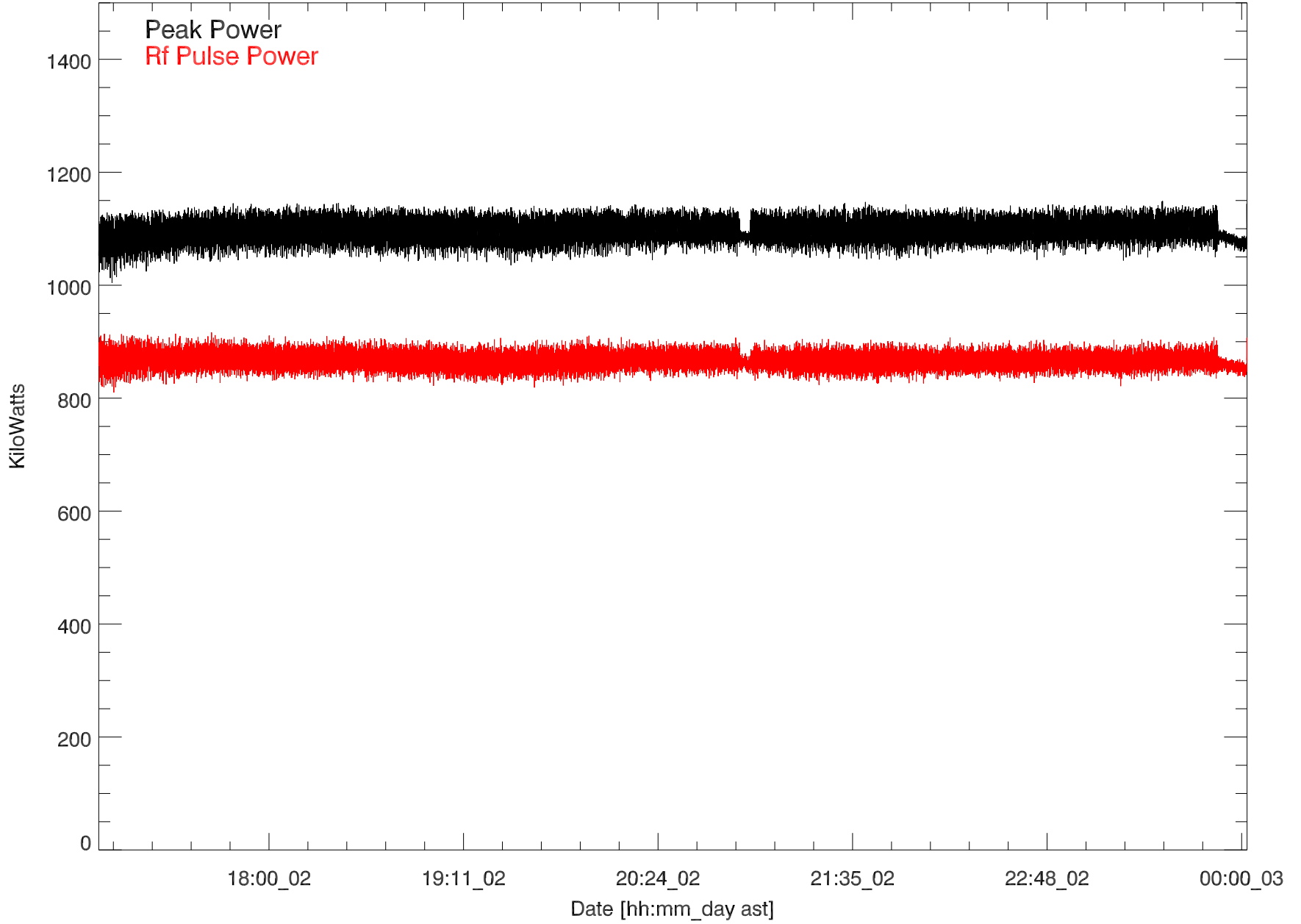
GD 430 Transmitted power for: 02nov18:H3255_5
