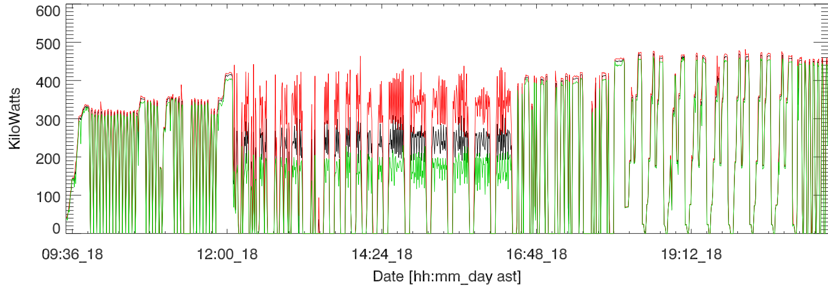
mar18 hf campaign, Transmitted power (total). 18mar
