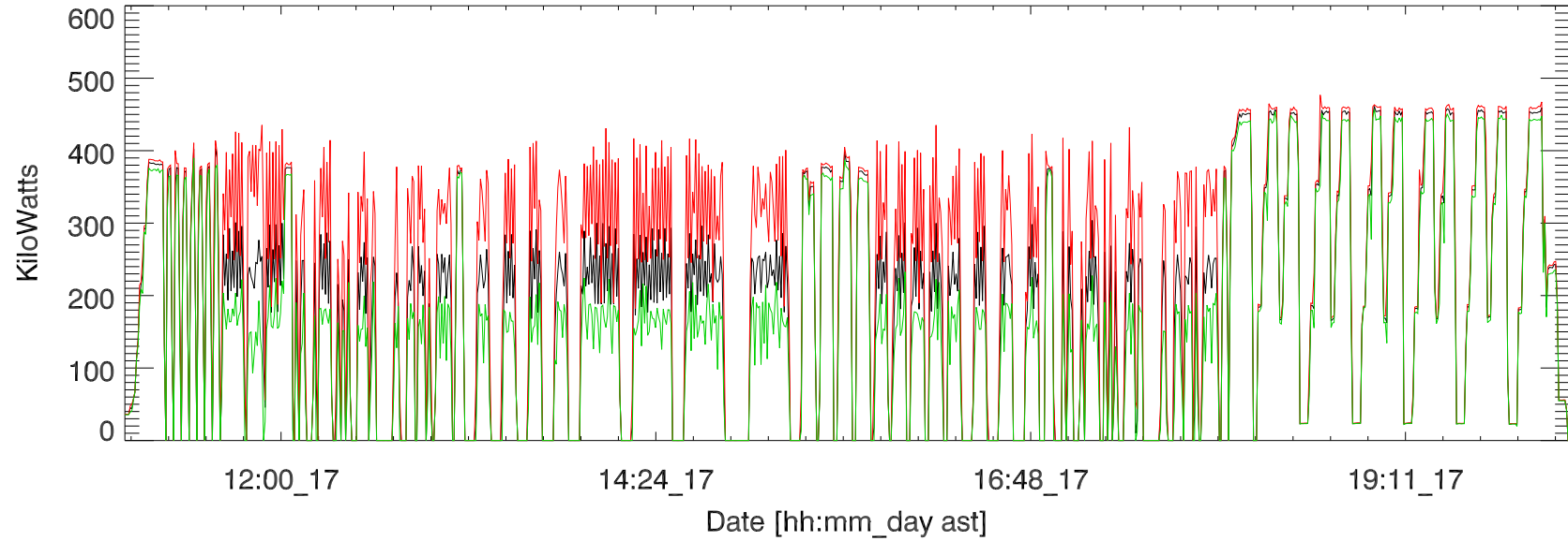
mar18 hf campaign, Transmitted power (total). 17mar
