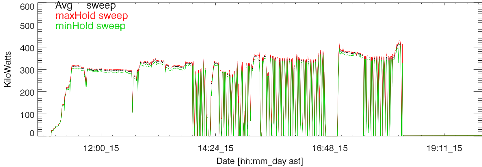
mar18 hf campaign, Transmitted power (total). 15mar
