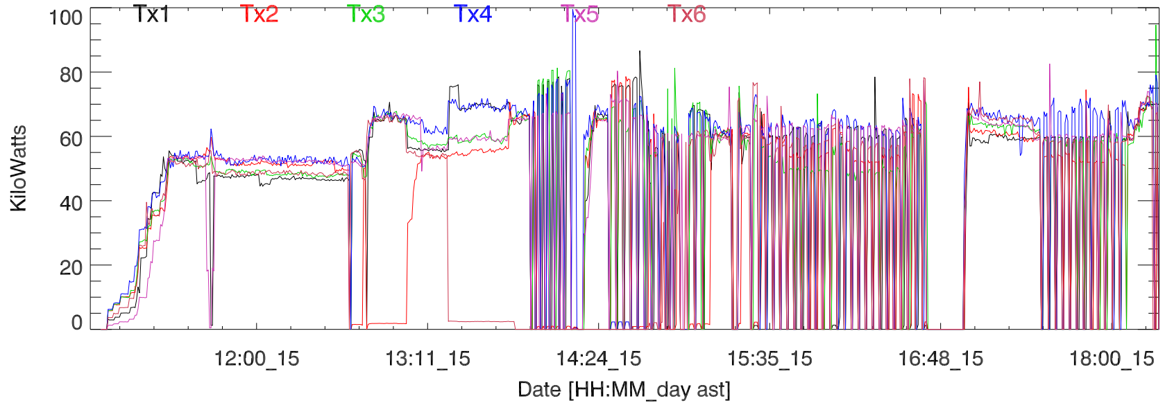
TxPwr by Tx. 15mar18:X115. HF TESTING
