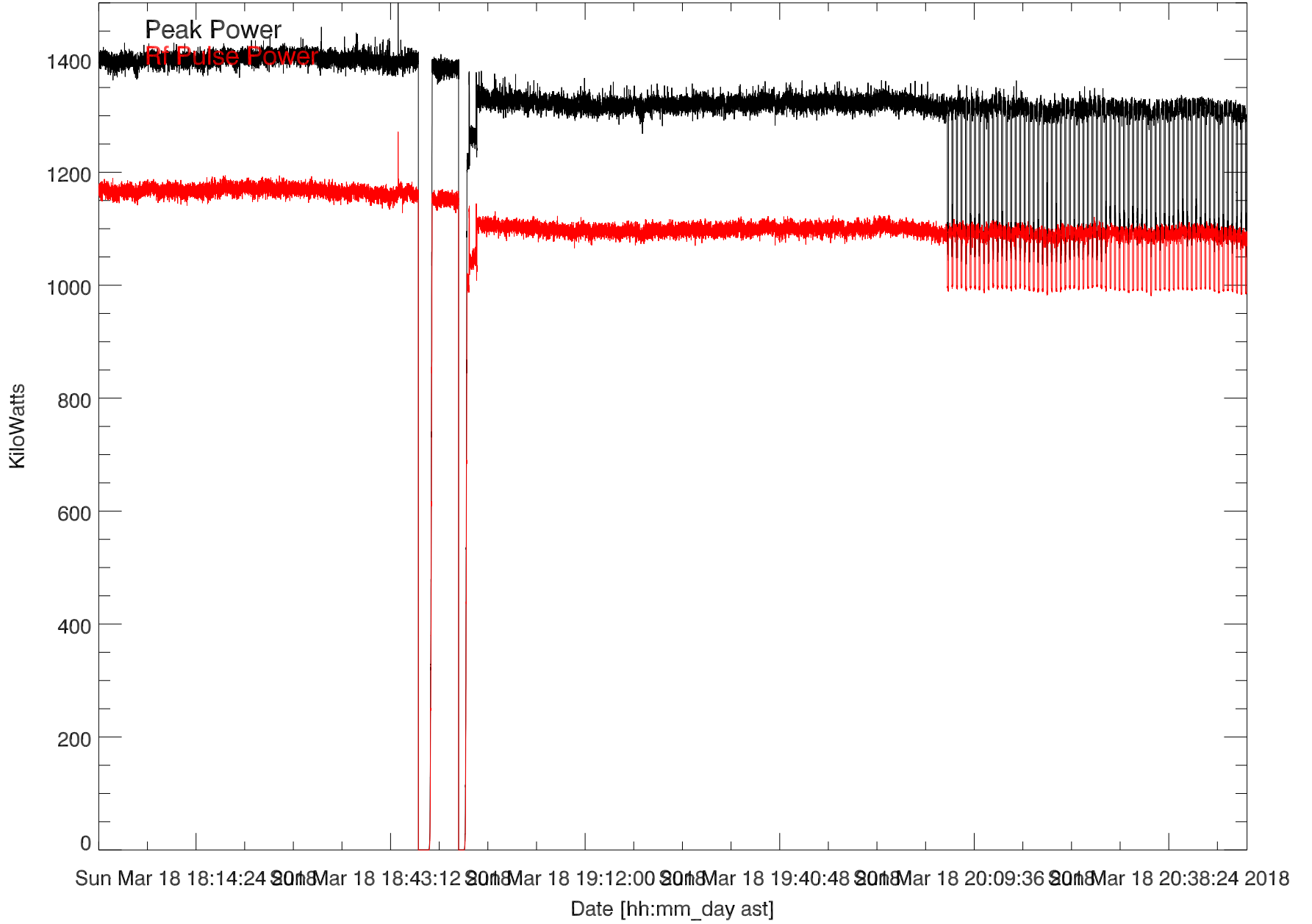
GD 430 Transmitted power for: 18mar18:H3249. Gennady
