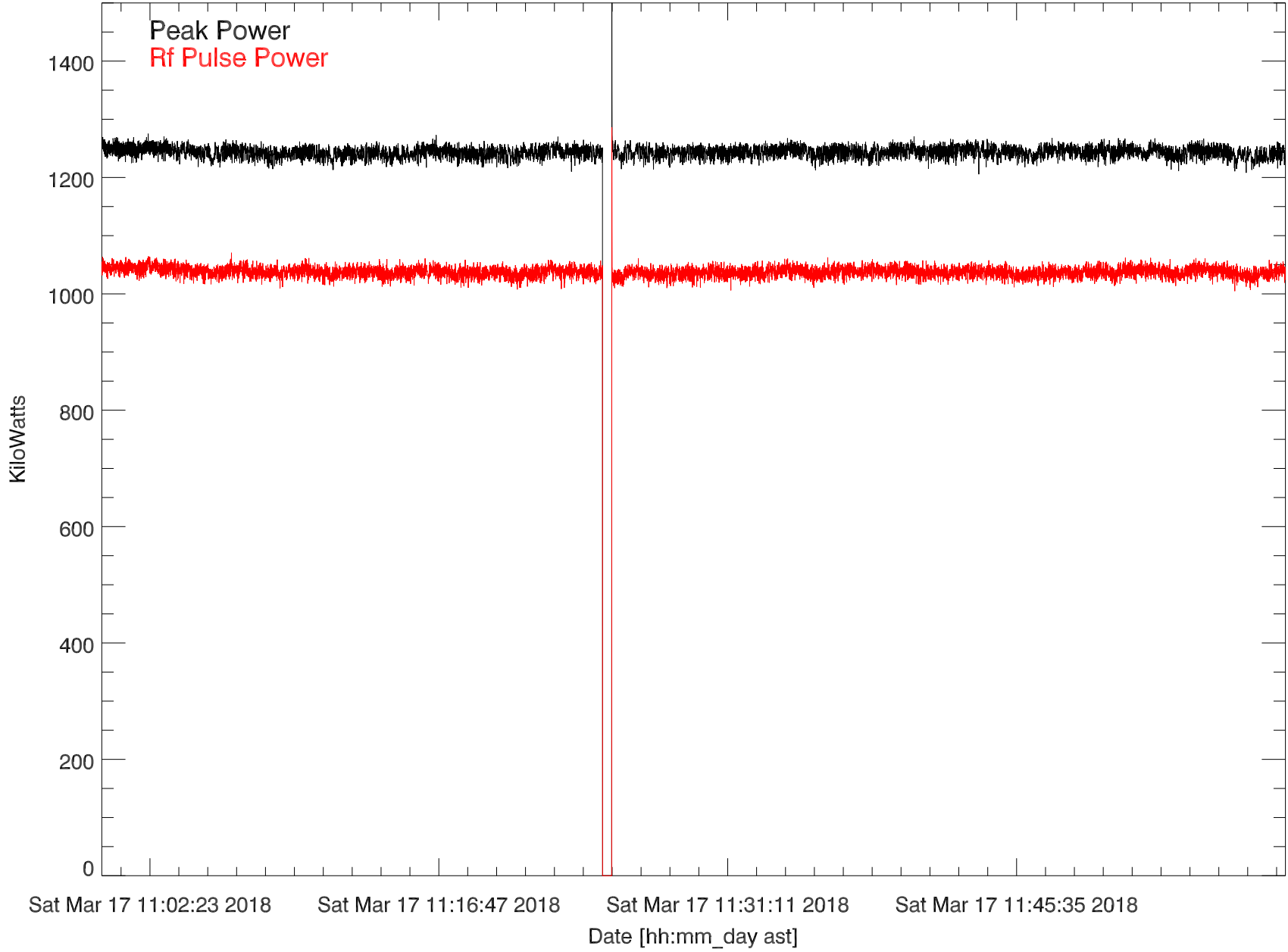
GD 430 Transmitted power for: 17mar18:X115 testing
