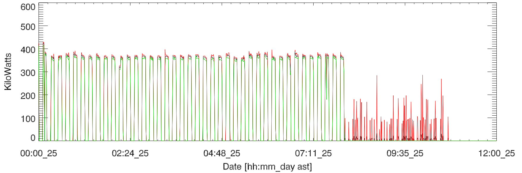
jul17 hf campaign, Transmitted power (total). 25jul
