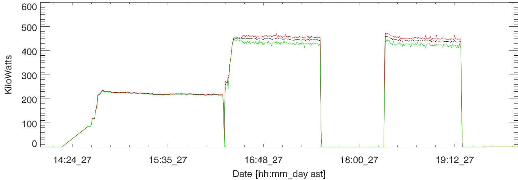
jul17 hf campaign, Transmitted power (total). 27jul
