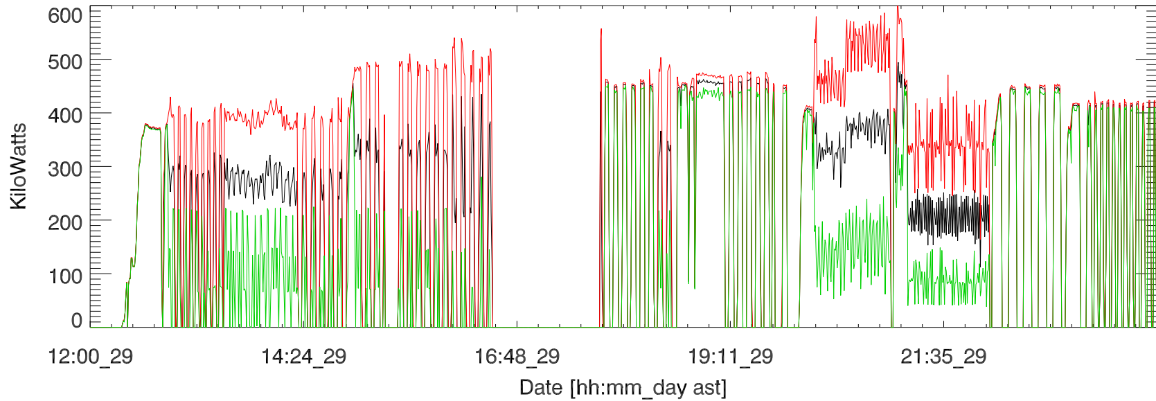
jul17 hf campaign, Transmitted power (total). 29jul
