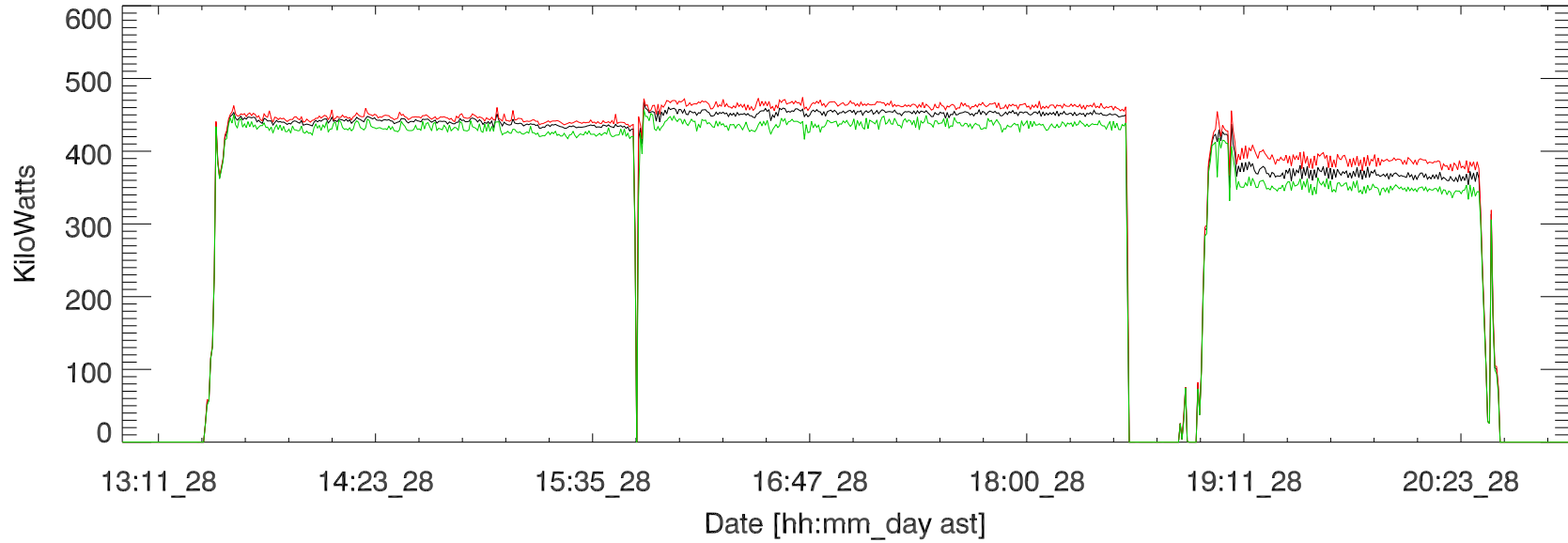
jul17 hf campaign, Transmitted power (total). 28jul
