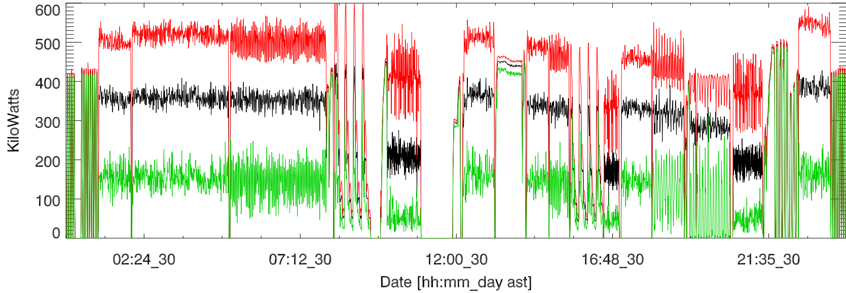
jul17 hf campaign, Transmitted power (total). 30jul
