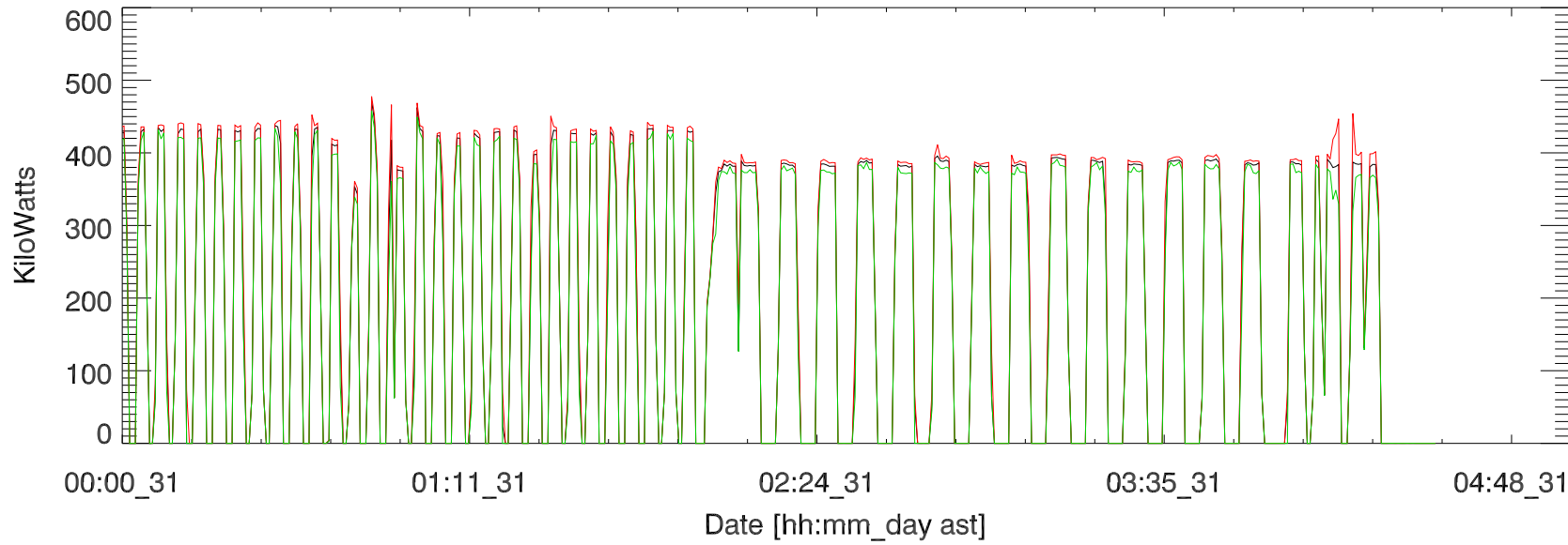
jul17 hf campaign, Transmitted power (total). 31jul
