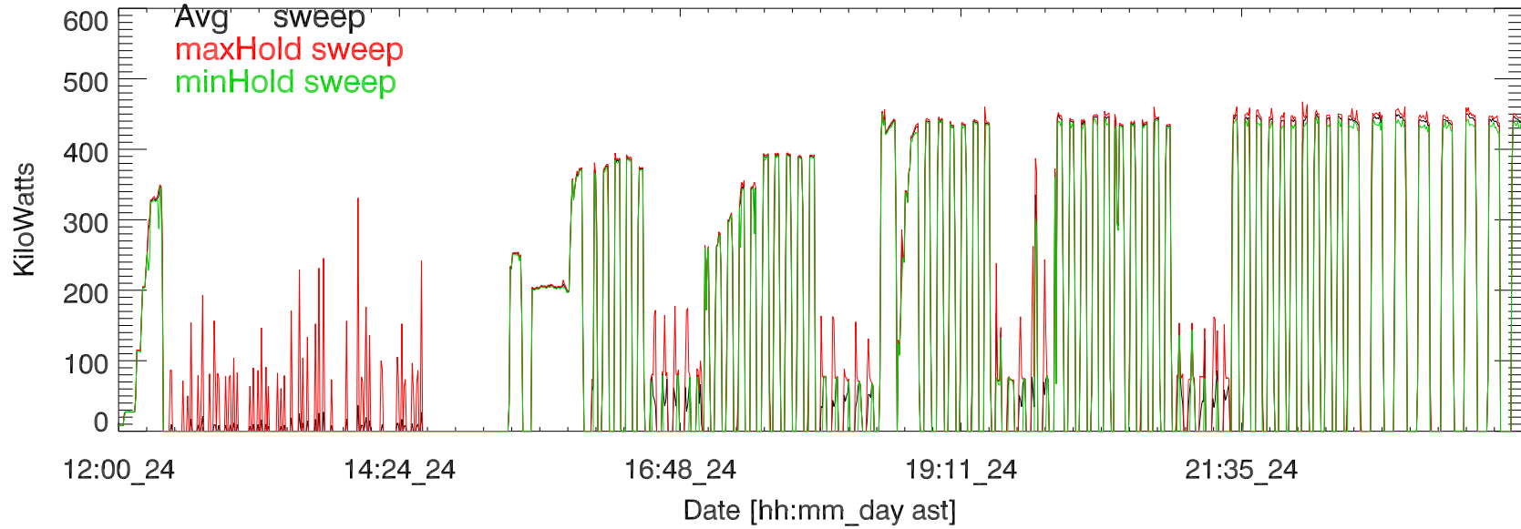
jul17 hf campaign, Transmitted power (total). 24jul
