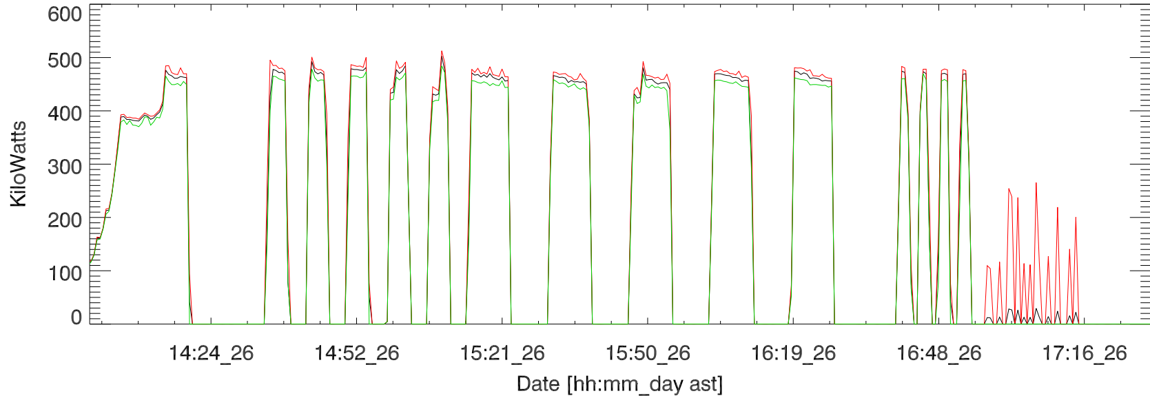
jul17 hf campaign, Transmitted power (total). 26jul
