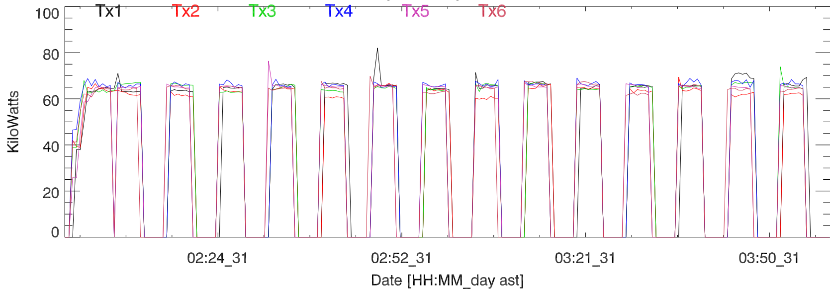
TxPwr by Tx. 31jul17: Andreas
