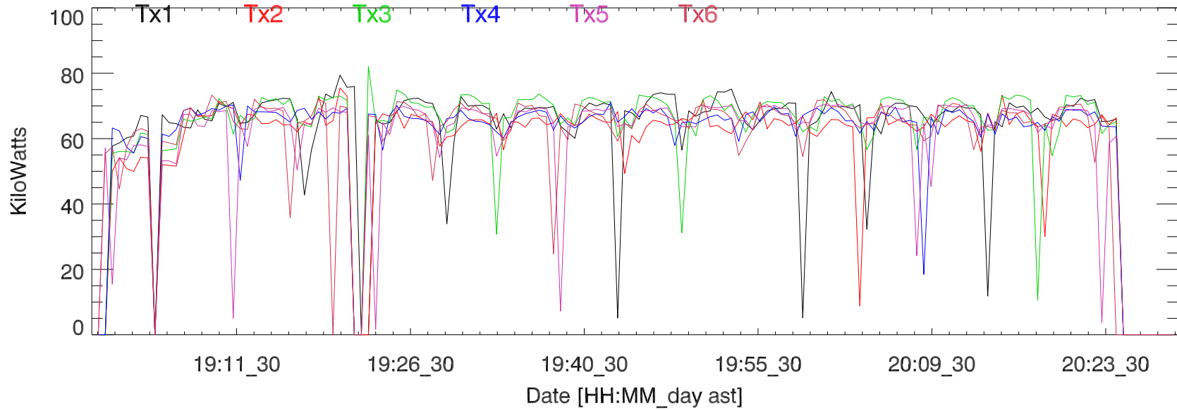
TxPwr by Tx. 30jul17: Hunter
