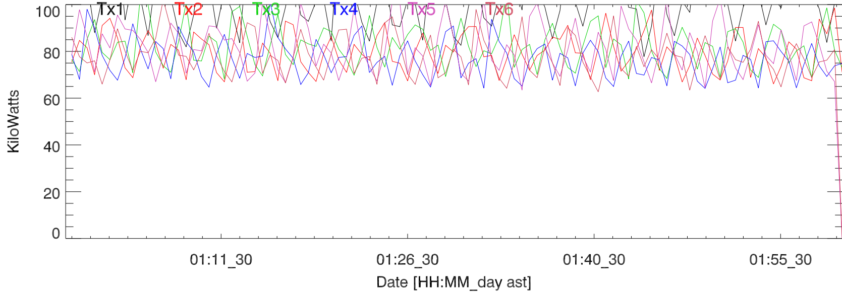
TxPwr by Tx. 30jul17: Quincy
