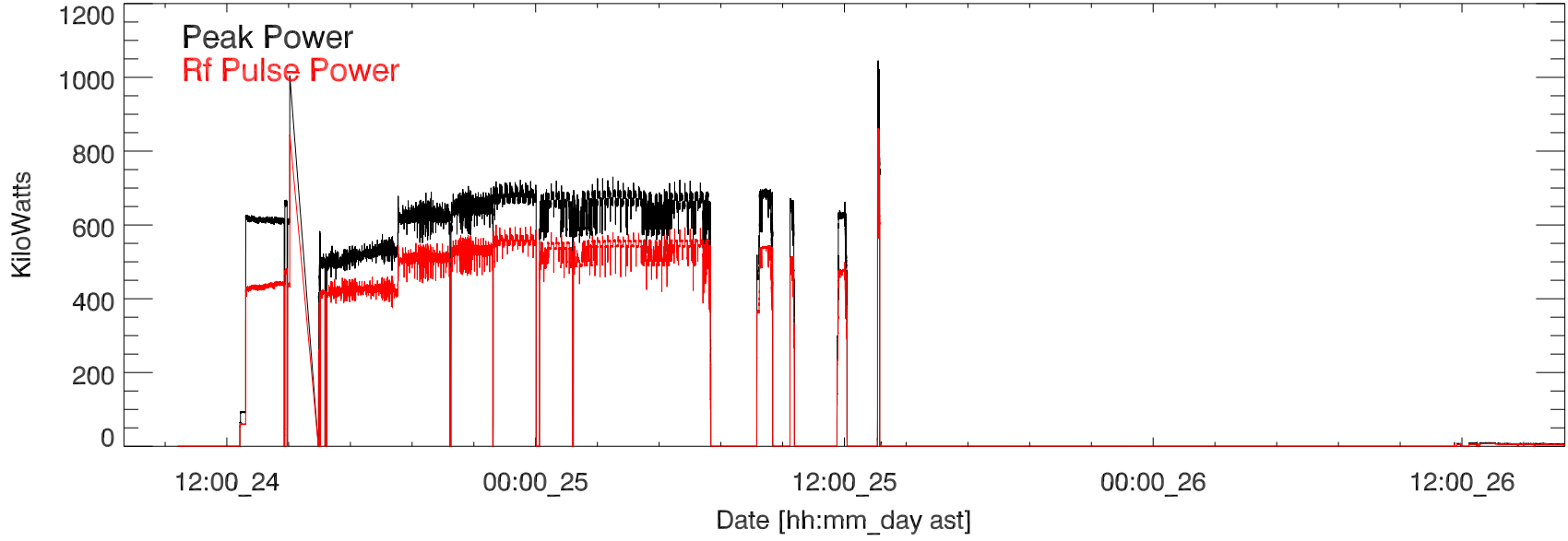
CH 430 Transmitted power for hf jul17
