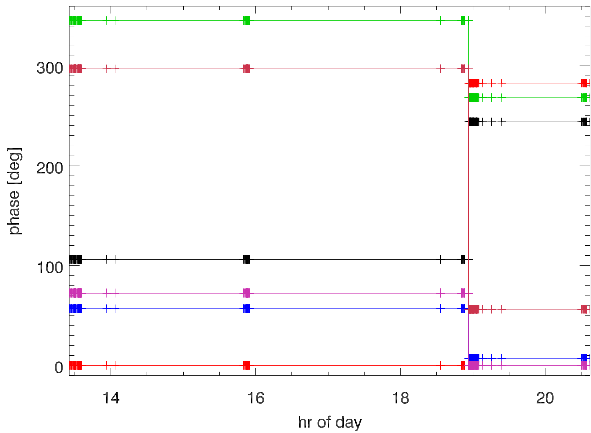
jul17 hf campaign 20170728 synth phase
