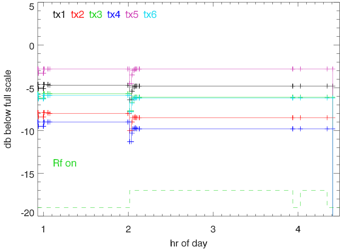
jul17 hf campaign 20170731 synth drive amplitude
