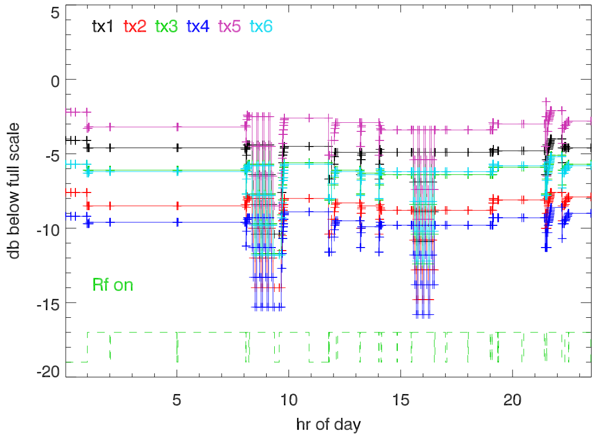
jul17 hf campaign 20170730 synth drive amplitude
