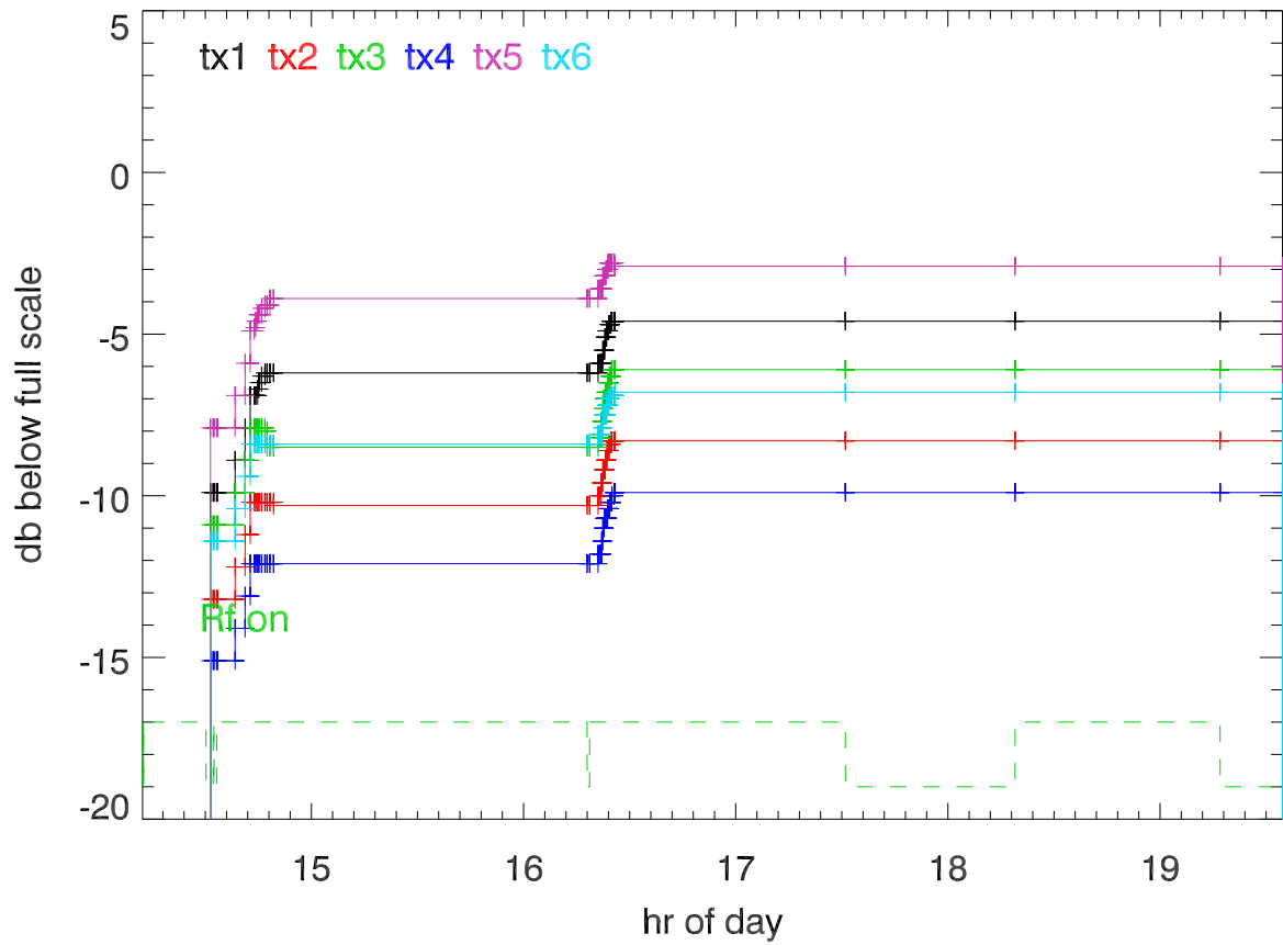
jul17 hf campaign 20170727 synth drive amplitude
