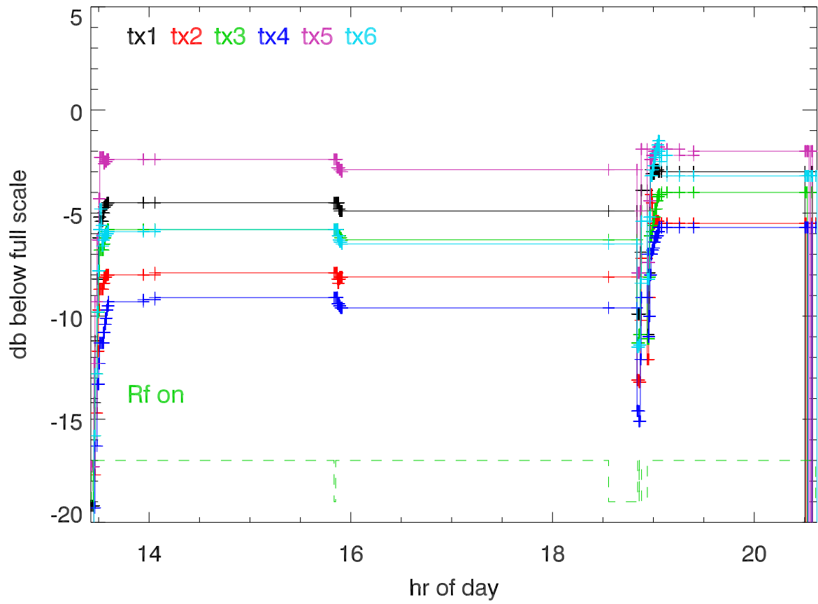
jul17 hf campaign 20170728 synth drive amplitude
