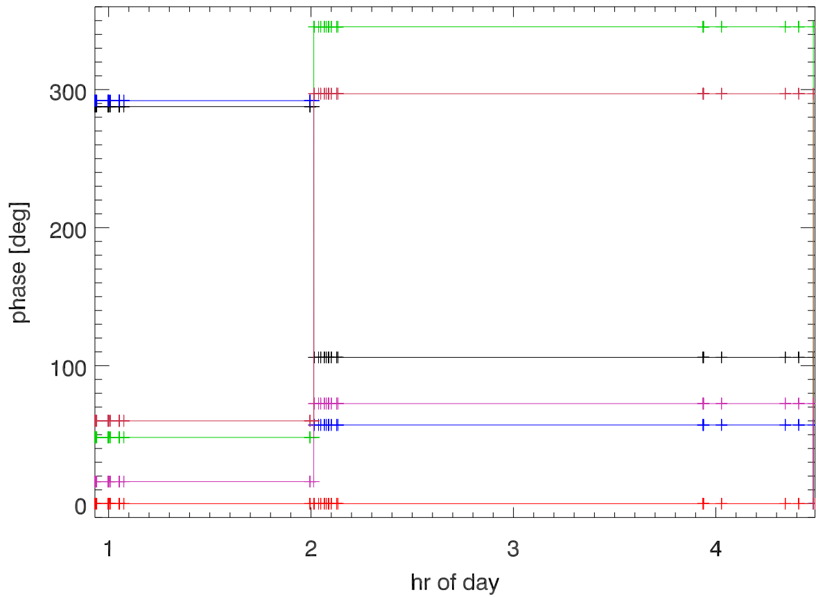
jul17 hf campaign 20170731 synth phase
