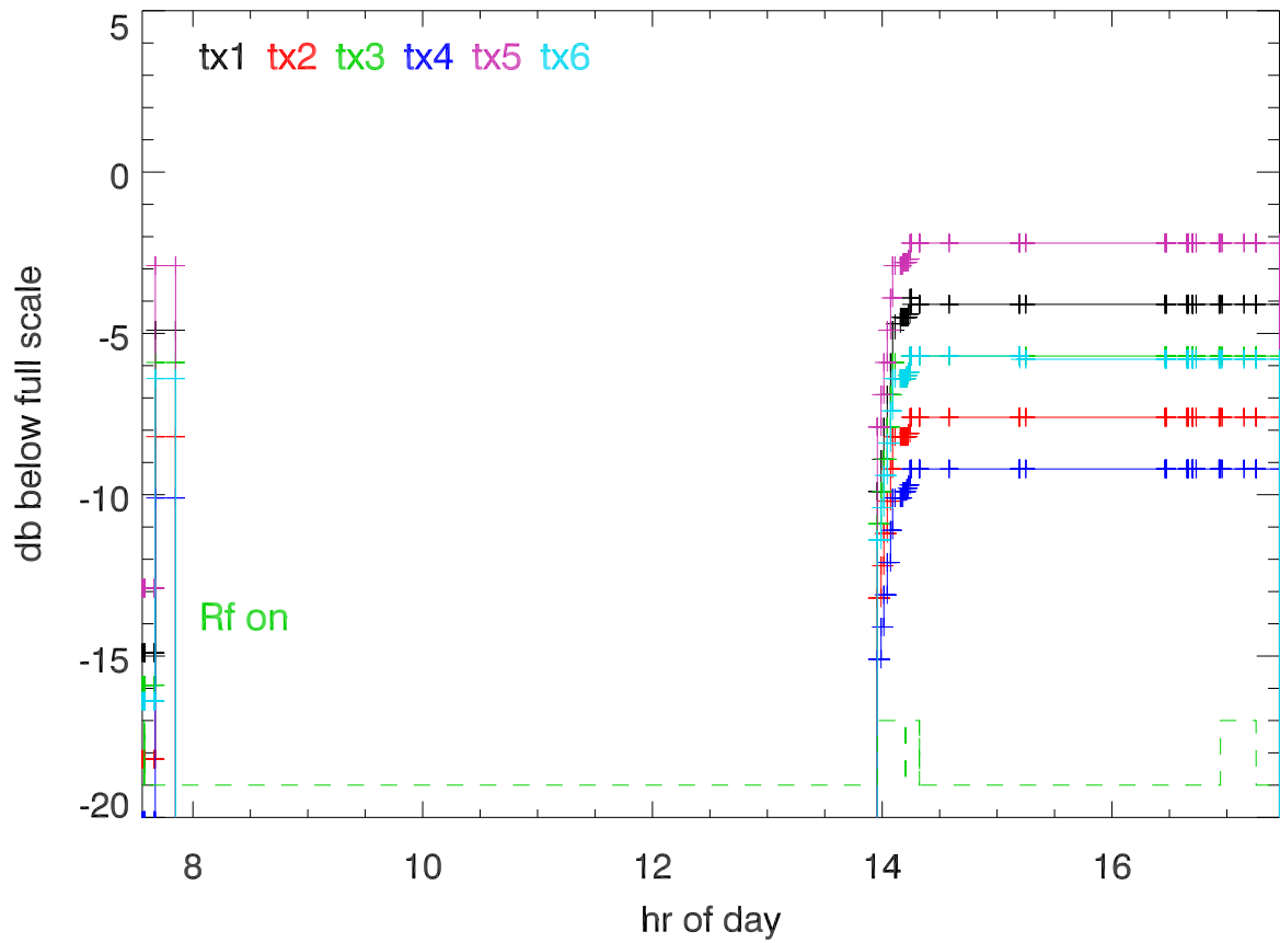
jul17 hf campaign 20170726 synth drive amplitude
