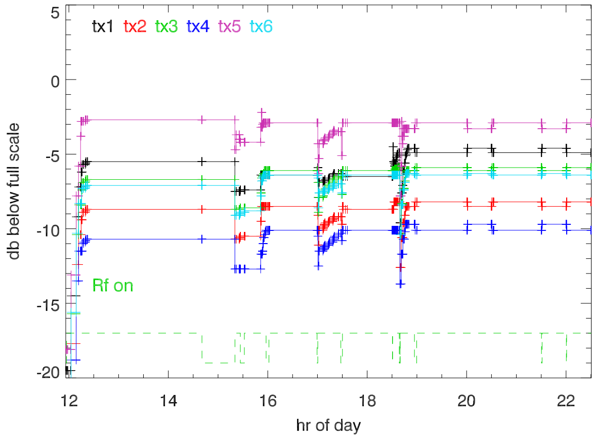
jul17 hf campaign 20170724 synth drive amplitude
