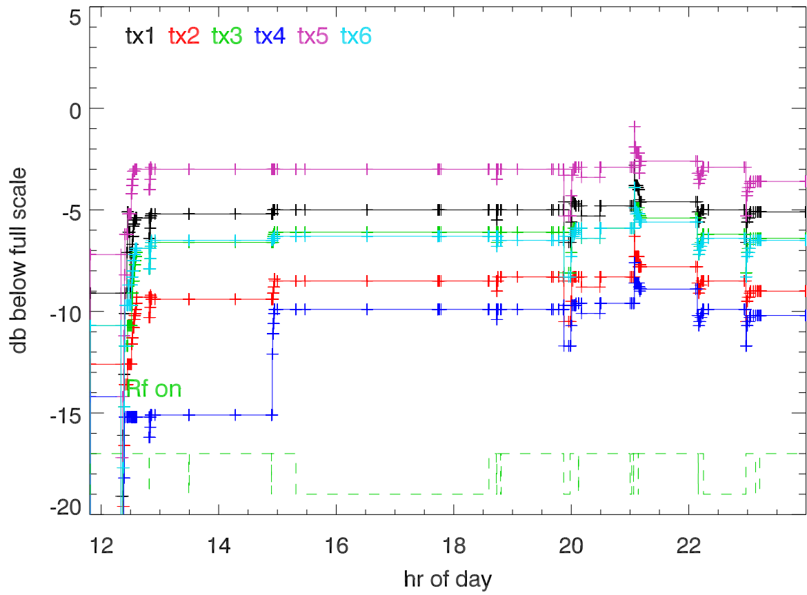
jul17 hf campaign 20170729 synth drive amplitude
