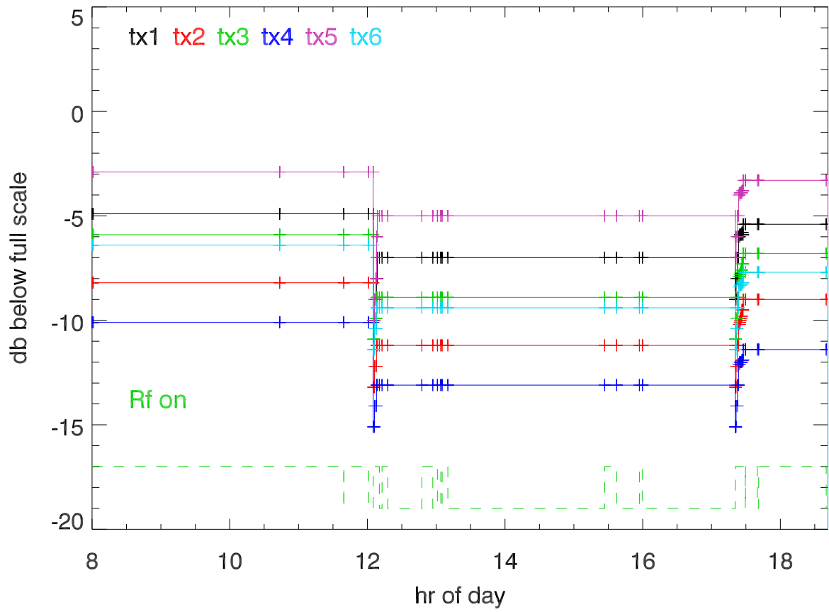
jul17 hf campaign 20170725 synth drive amplitude
