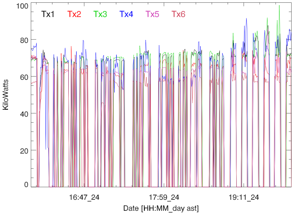
TxPwr by Tx. 24may17:H3194. Natasha Jackson-Booth
