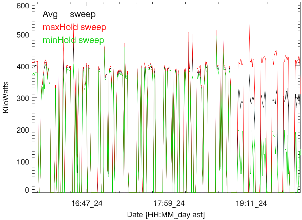
TxPwrTot. 24may17:H3194. Natasha Jackson-Booth8 MHz
