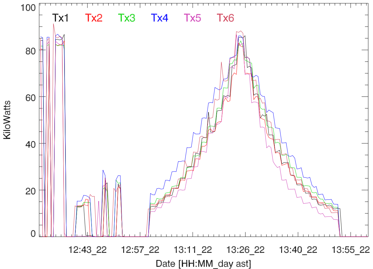
TxPwr by Tx. 22may17:H3171. Eliana Nossa.
