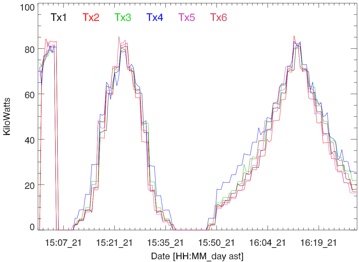
TxPwr by Tx. 21may17:H3171. Eliana Nossa.
