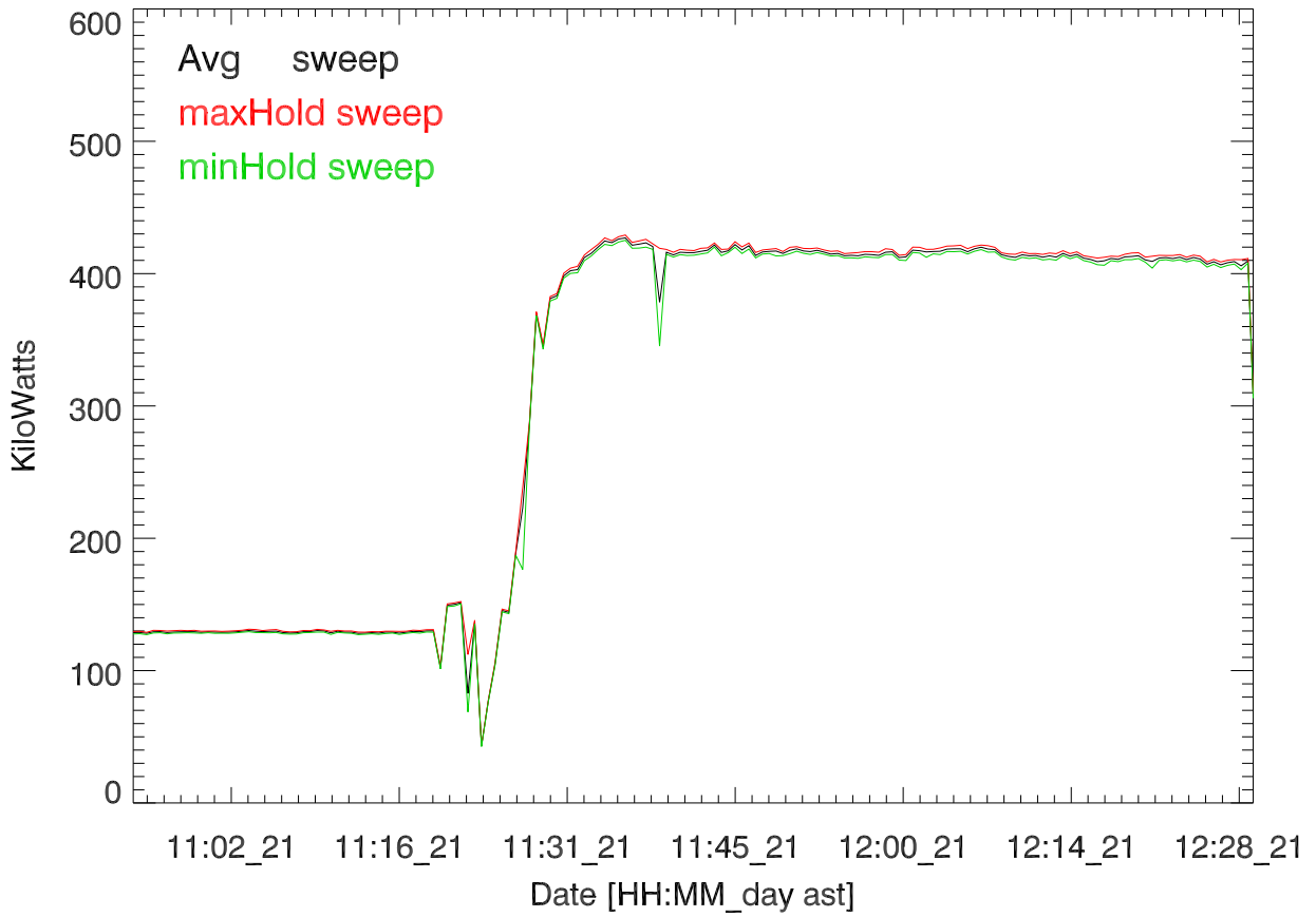
TxPwrTot. 21may17:H3156. Paul Bernhardt 5 MHz
