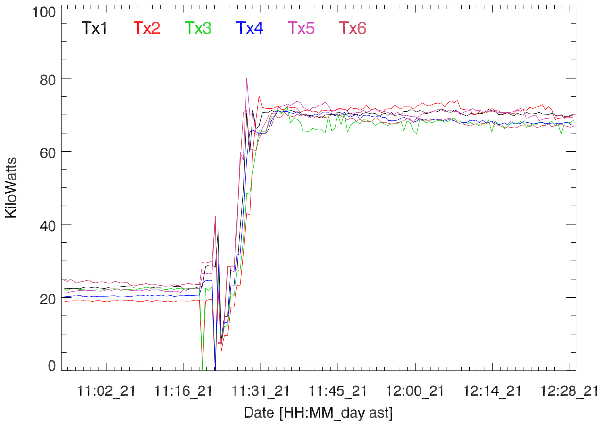
TxPwr by Tx. 21may17:H3156. Paul Bernhardt
