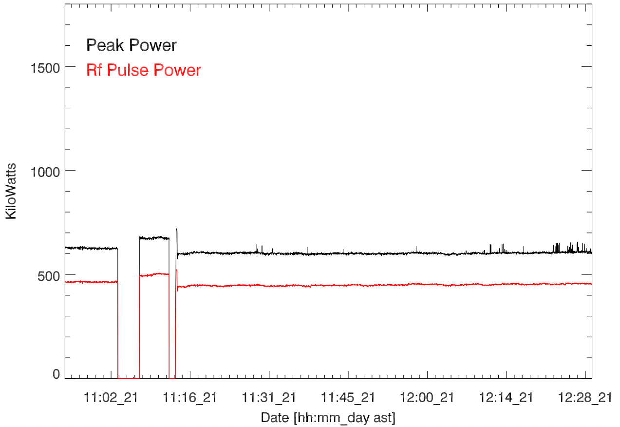
CH 430 Transmitted power for: 21may17:H3156. Paul Bernhardt
