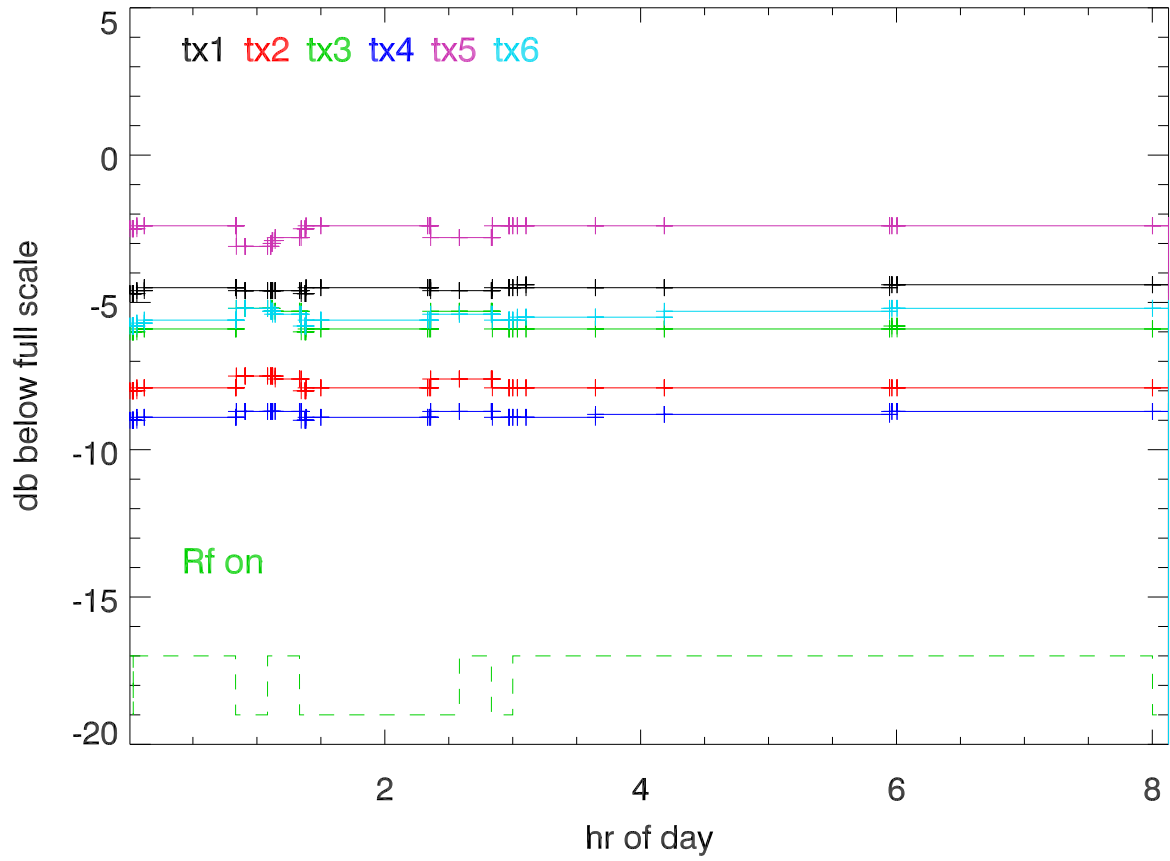
may17 hf campaign 20170526 synth drive amplitude
