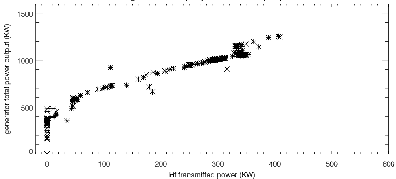
generator output power vs hf output pwr
