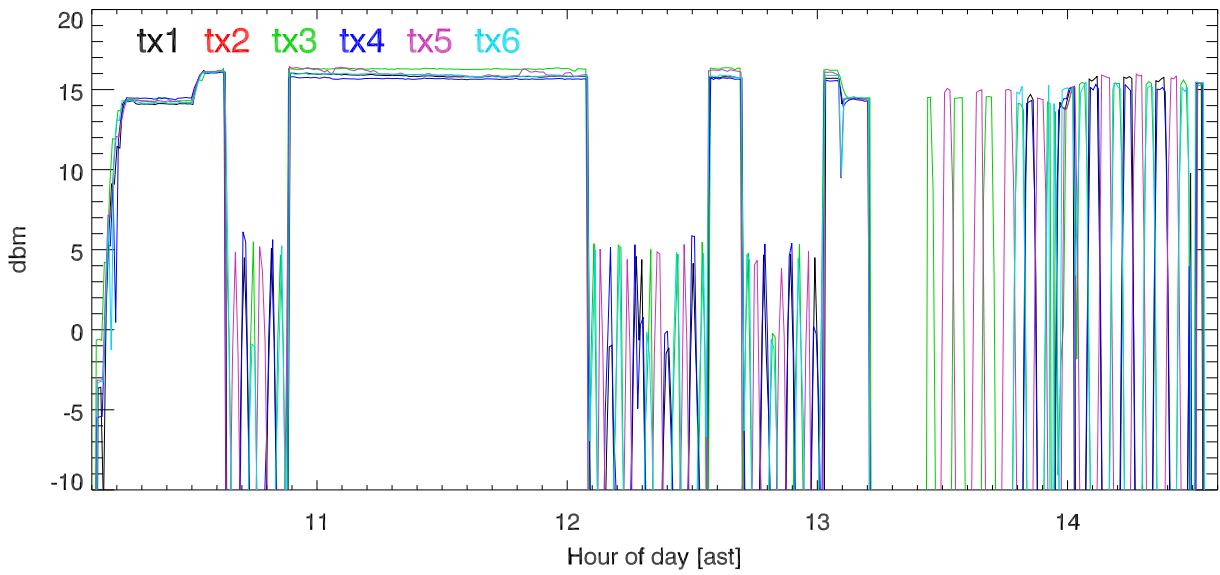
190603 5 MHz Band tx power. rf coupler output. . 5 Mhz test.
