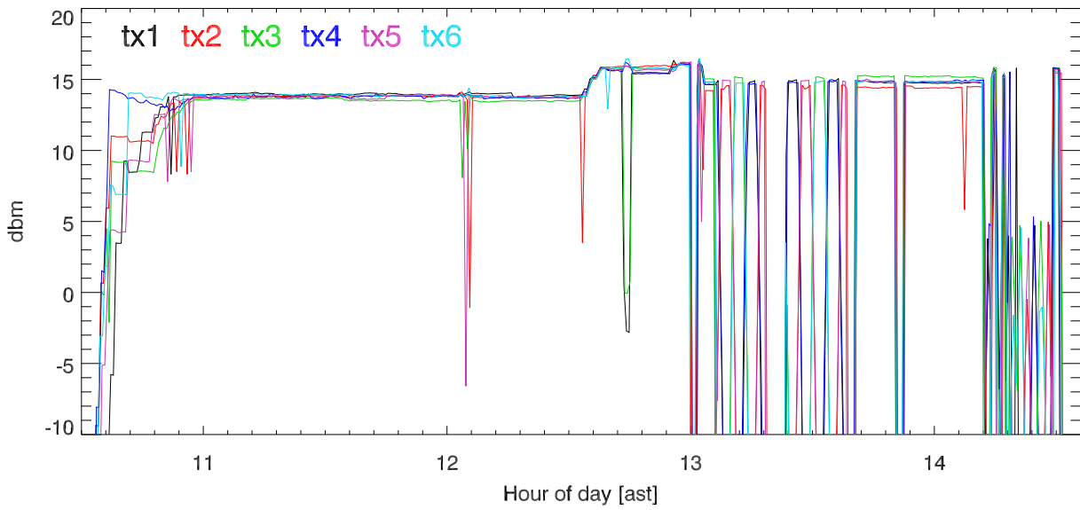
190522 5 MHz Band tx power. rf coupler output. . 8Mhz test.
