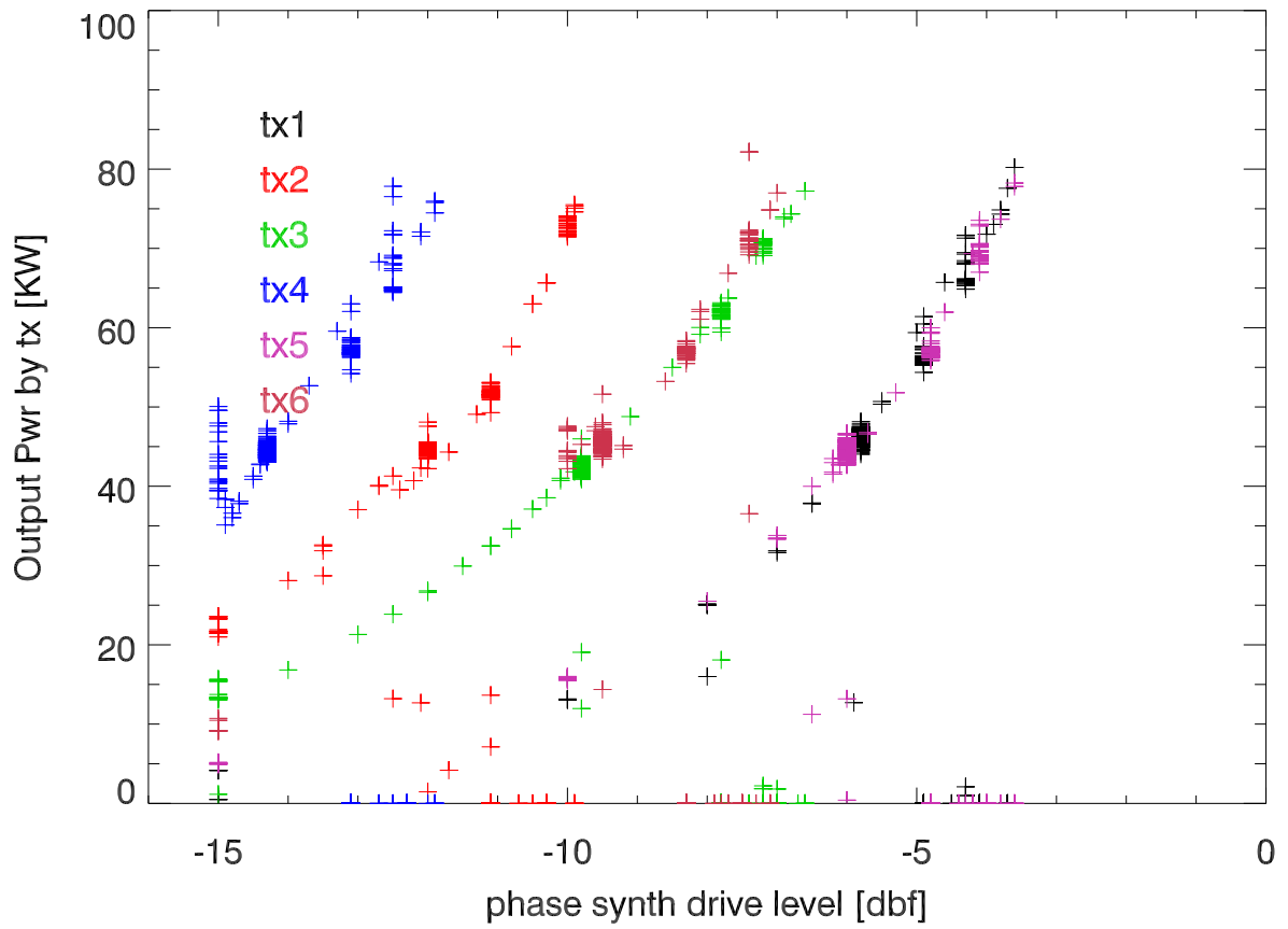
190522 HF output Power vs drive level
