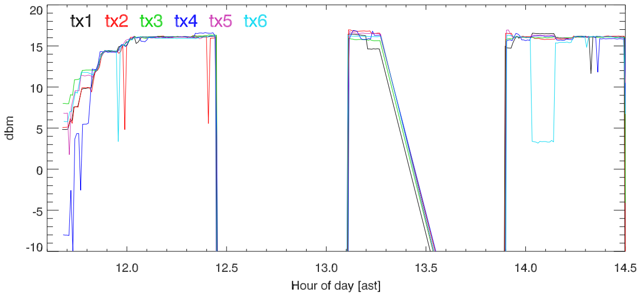
190509 5 MHz Band tx power. rf coupler output. . 8Mhz test.
