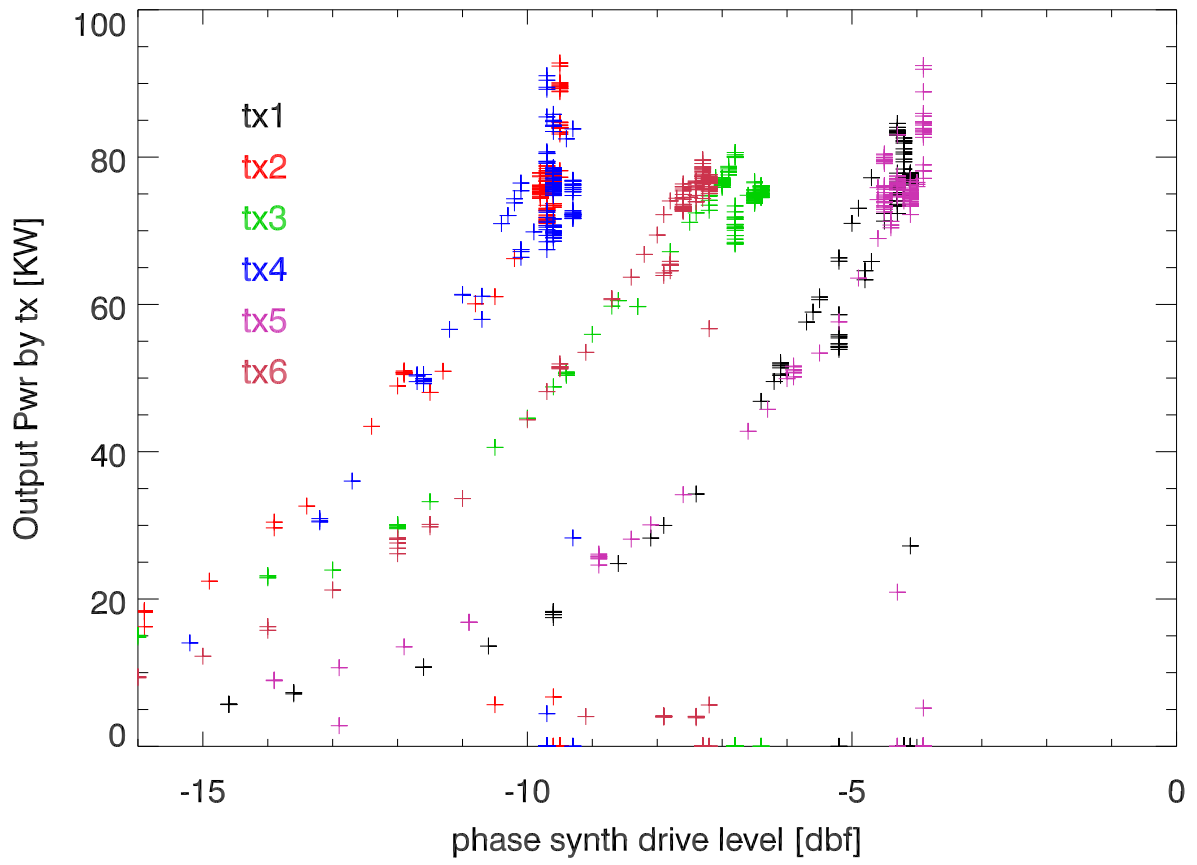
190509 HF output Power vs drive level
