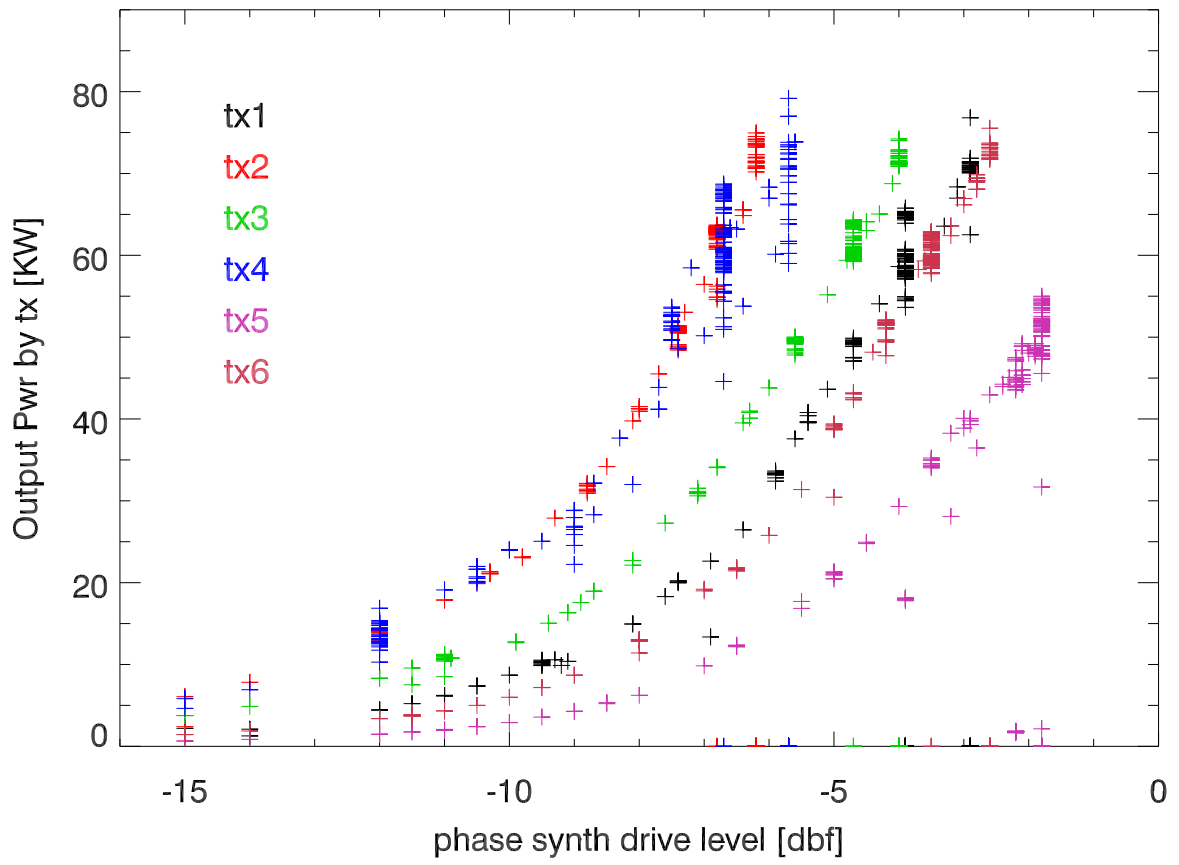
180926 HF output Power vs drive level
