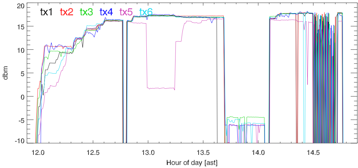
180926 8 Mhz Band tx power. rf coupler output. . 8Mhz test.
