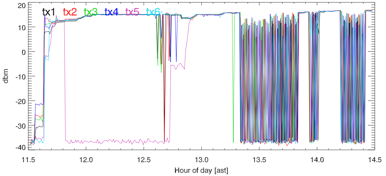
180919 5 MHz Band tx power. rf coupler output. . 5Mhz test.
