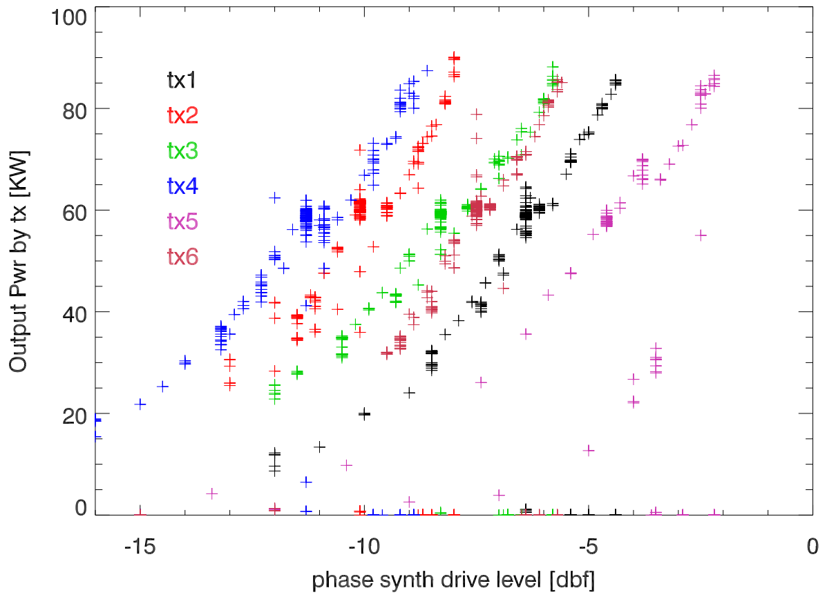
180919 HF output Power vs drive level
