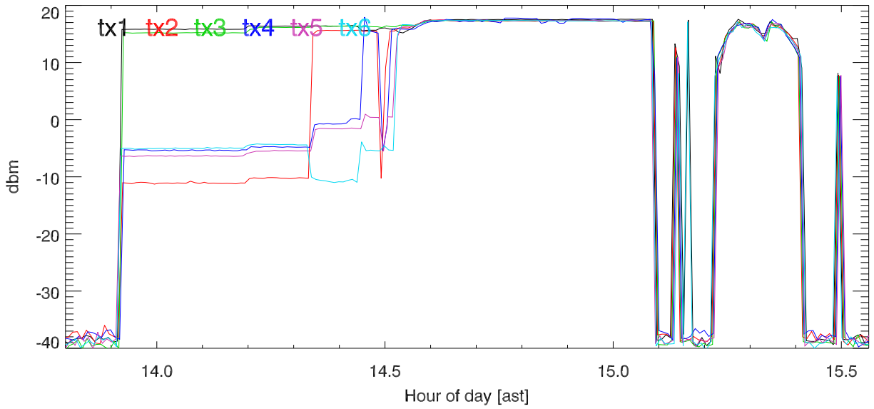
170301 8 Mhz Band tx power. rf coupler output. . 8Mhz test.
