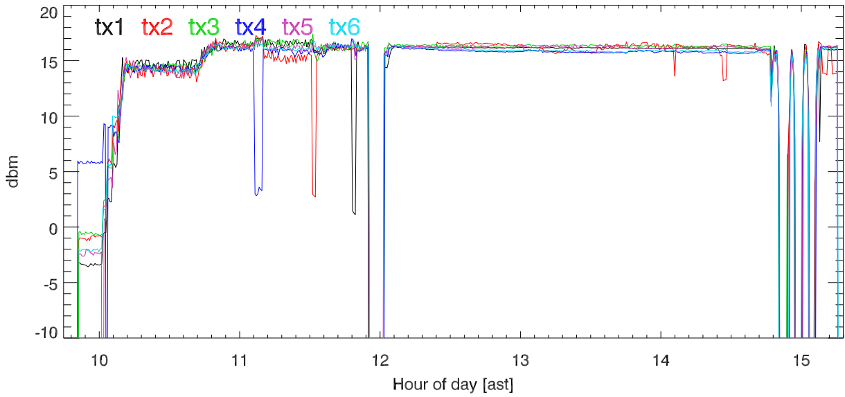
170214 5 MHz Band tx power. rf coupler output. . 5Mhz test.
