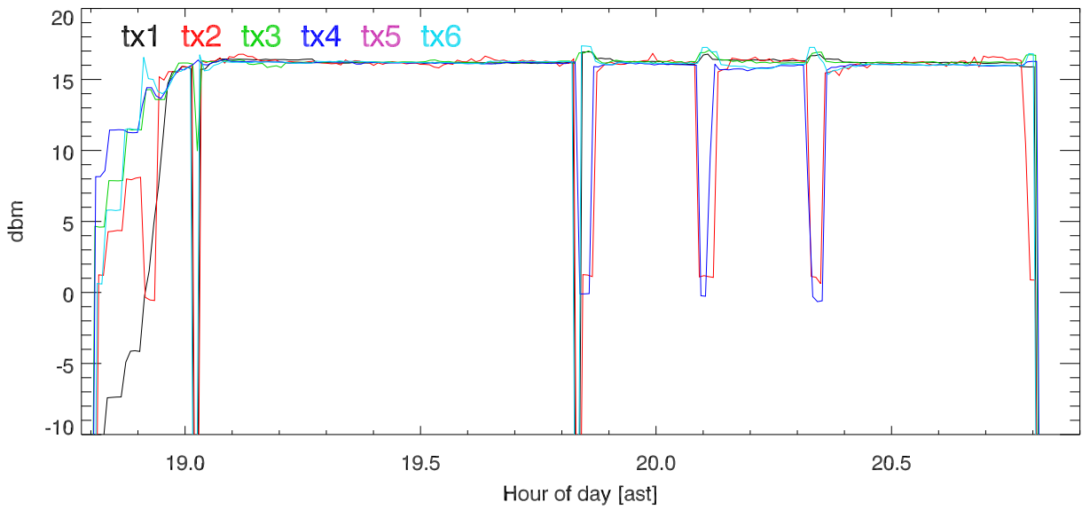
170126 5 MHz Band tx power. rf coupler output. . 5Mhz test. set 2
