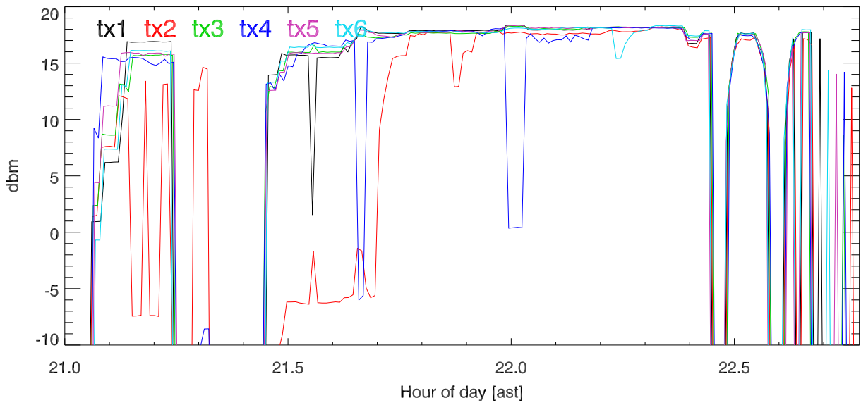
170126 8 Mhz Band tx power. rf coupler output. . 8 MHz test
