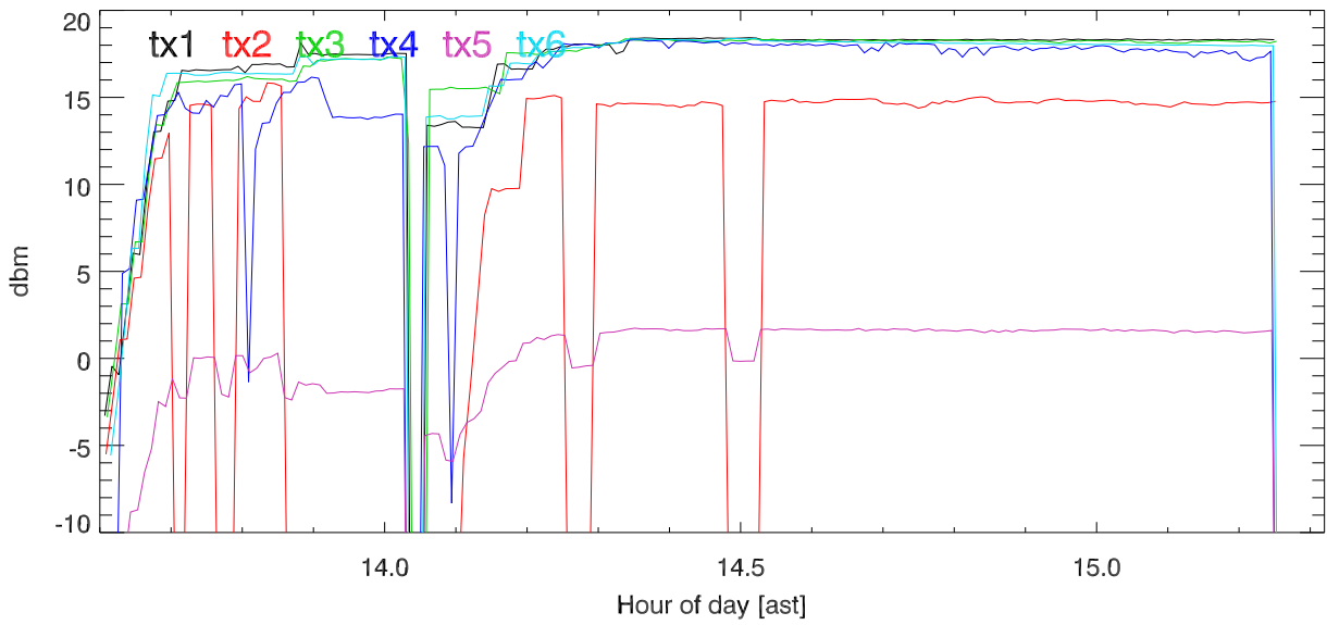
170118 8 Mhz Band tx power. rf coupler output. . Center of dish covered
