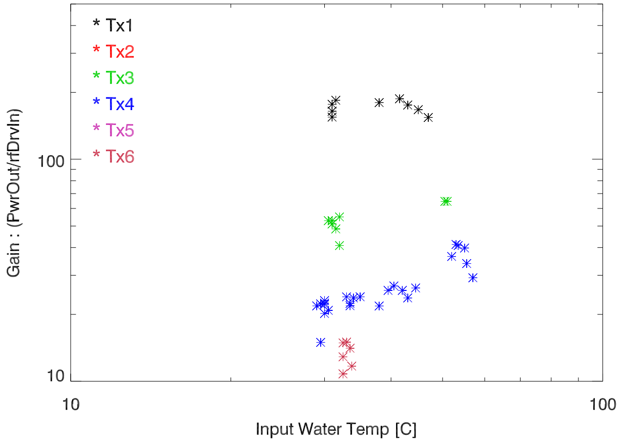
hf: tx gain vs input water temp
