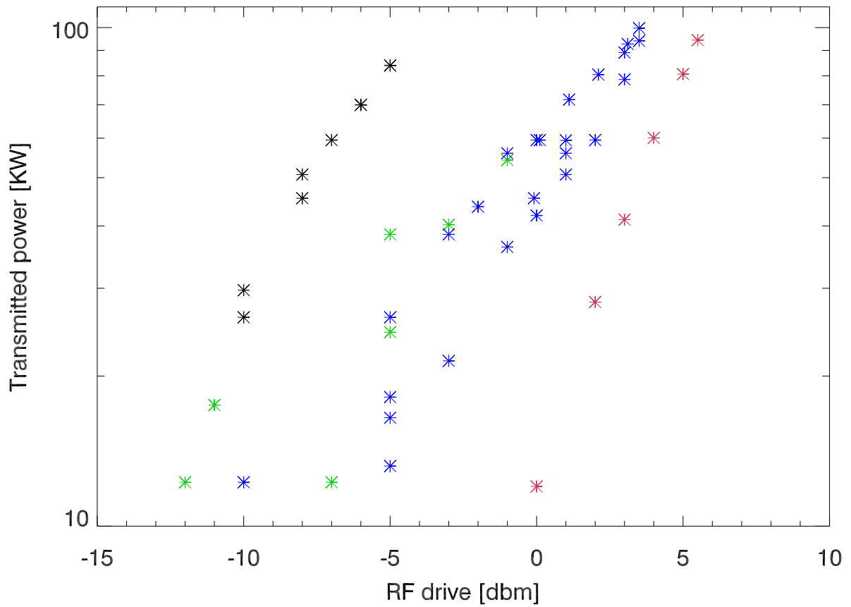
hf: Transmitted power vs rf drive input
