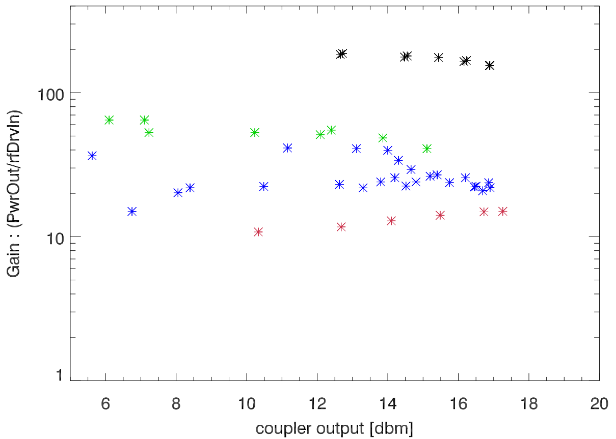
hf: tx gain vs outputPwr
