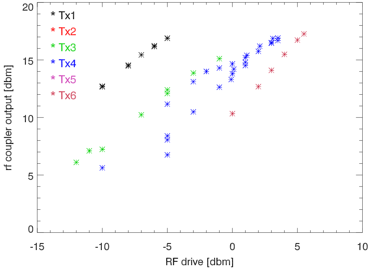
hf: rf coupler output vs rf drive input
