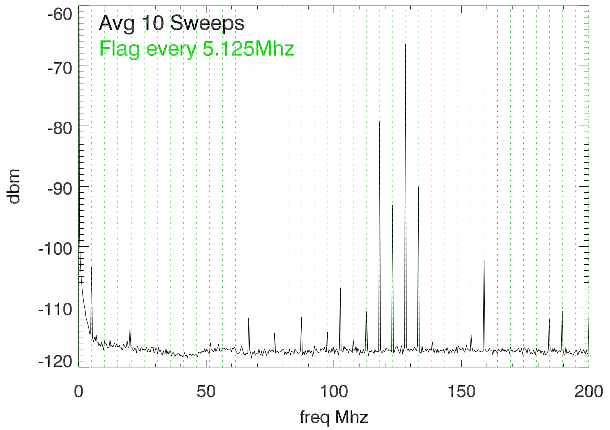
06may15 75Mhz hipass filter. blowup 0-200 MHz
