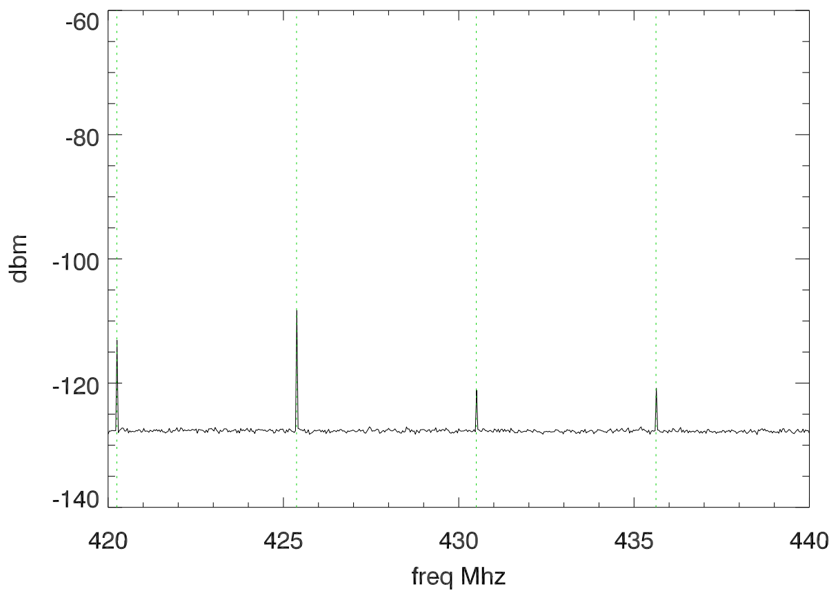
20 Mhz about 430 Mhz. 1KHz rbw
