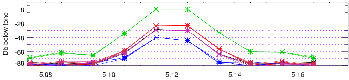
Harmonic Levels relative to tone power. Tone pwr: 9.8 KW
