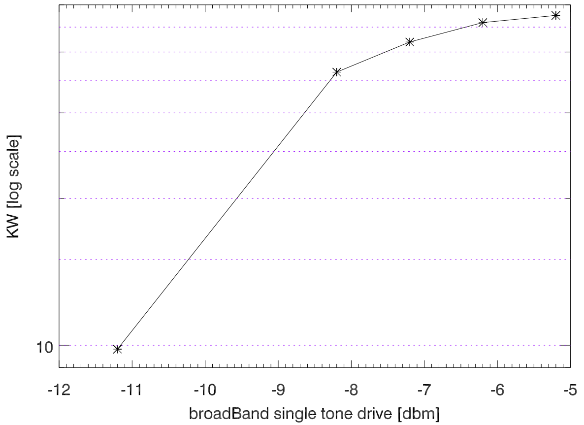
190509 Single Tone output power vs drvPower
